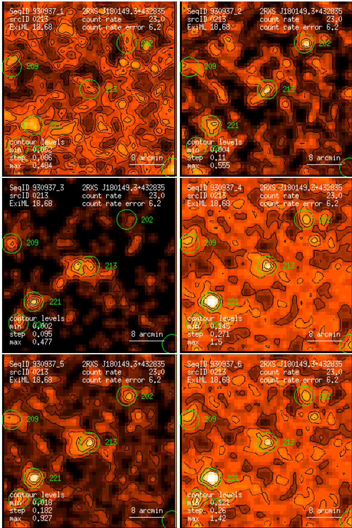
Figure 213: RASS 930937: detection 0213: band rate images, Gaussian filter: (1) PSPC channels 11 – 41, (2) 52 – 90, (3) 91 – 201, (4) 11 – 235, (5) 52 – 201, (6) 11 – 201. Broad band rates in counts/ks. Band rate contour levels in counts/ks/arcmin 2 .
