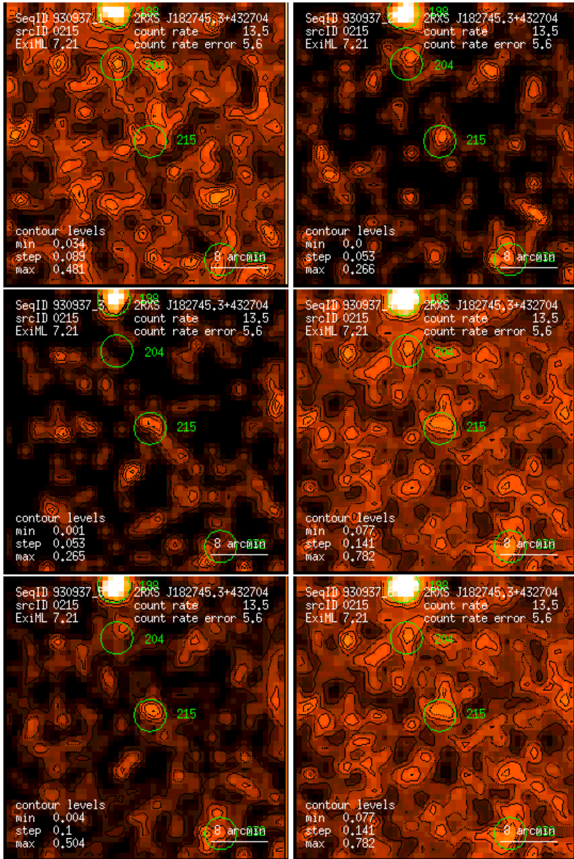
Figure 215: RASS 930937: detection 0215: band rate images, Gaussian filter: (1) PSPC channels 11 – 41, (2) 52 – 90, (3) 91 – 201, (4) 11 – 235, (5) 52 – 201, (6) 11 – 201. Broad band rates in counts/ks. Band rate contour levels in counts/ks/arcmin 2 .
