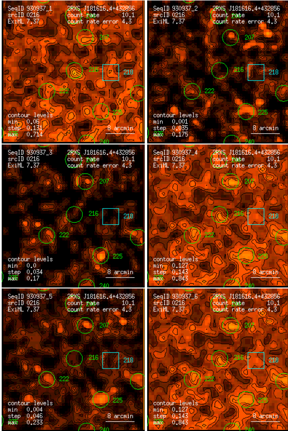
Figure 216: RASS 930937: detection 0216: band rate images, Gaussian filter: (1) PSPC channels 11 – 41, (2) 52 – 90, (3) 91 – 201, (4) 11 – 235, (5) 52 – 201, (6) 11 – 201. Broad band rates in counts/ks. Band rate contour levels in counts/ks/arcmin 2 .
