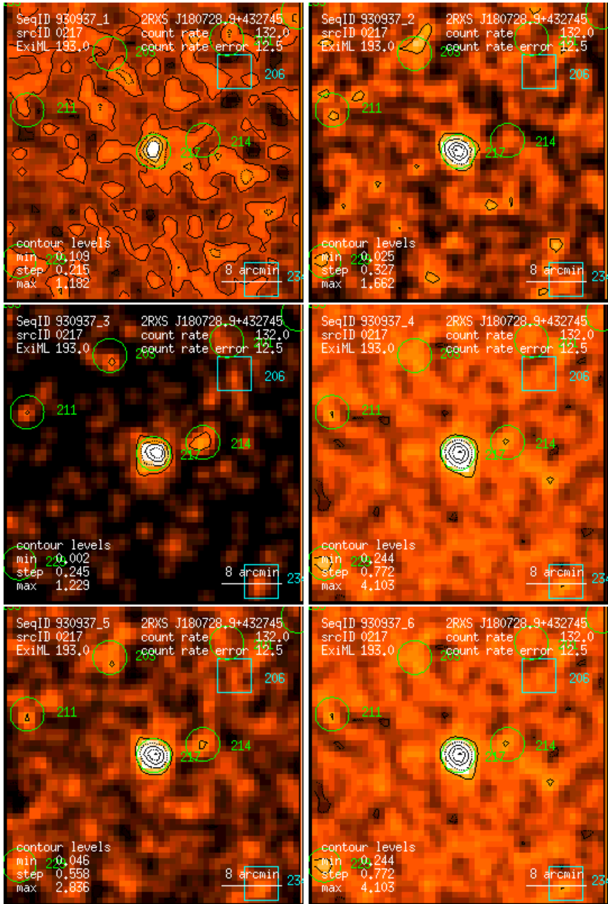
Figure 217: RASS 930937: detection 0217: band rate images, Gaussian filter: (1) PSPC channels 11 – 41, (2) 52 – 90, (3) 91 – 201, (4) 11 – 235, (5) 52 – 201, (6) 11 – 201. Broad band rates in counts/ks. Band rate contour levels in counts/ks/arcmin 2 .
