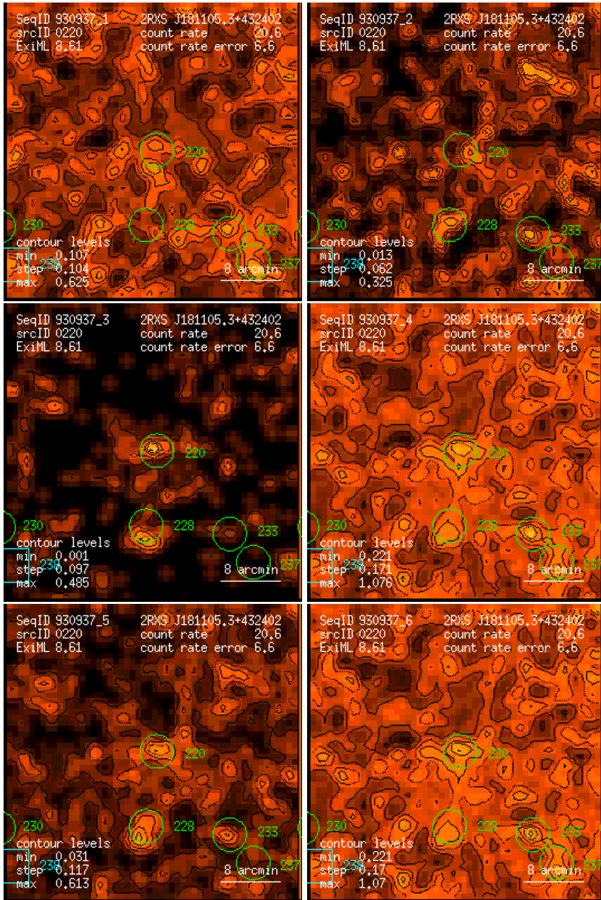
Figure 220: RASS 930937: detection 0220: band rate images, Gaussian filter: (1) PSPC channels 11 – 41, (2) 52 – 90, (3) 91 – 201, (4) 11 – 235, (5) 52 – 201, (6) 11 – 201. Broad band rates in counts/ks. Band rate contour levels in counts/ks/arcmin 2 .
