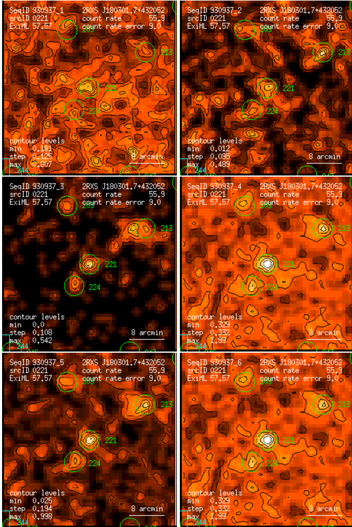
Figure 221: RASS 930937: detection 0221: band rate images, Gaussian filter: (1) PSPC channels 11 – 41, (2) 52 – 90, (3) 91 – 201, (4) 11 – 235, (5) 52 – 201, (6) 11 – 201. Broad band rates in counts/ks. Band rate contour levels in counts/ks/arcmin 2 .
