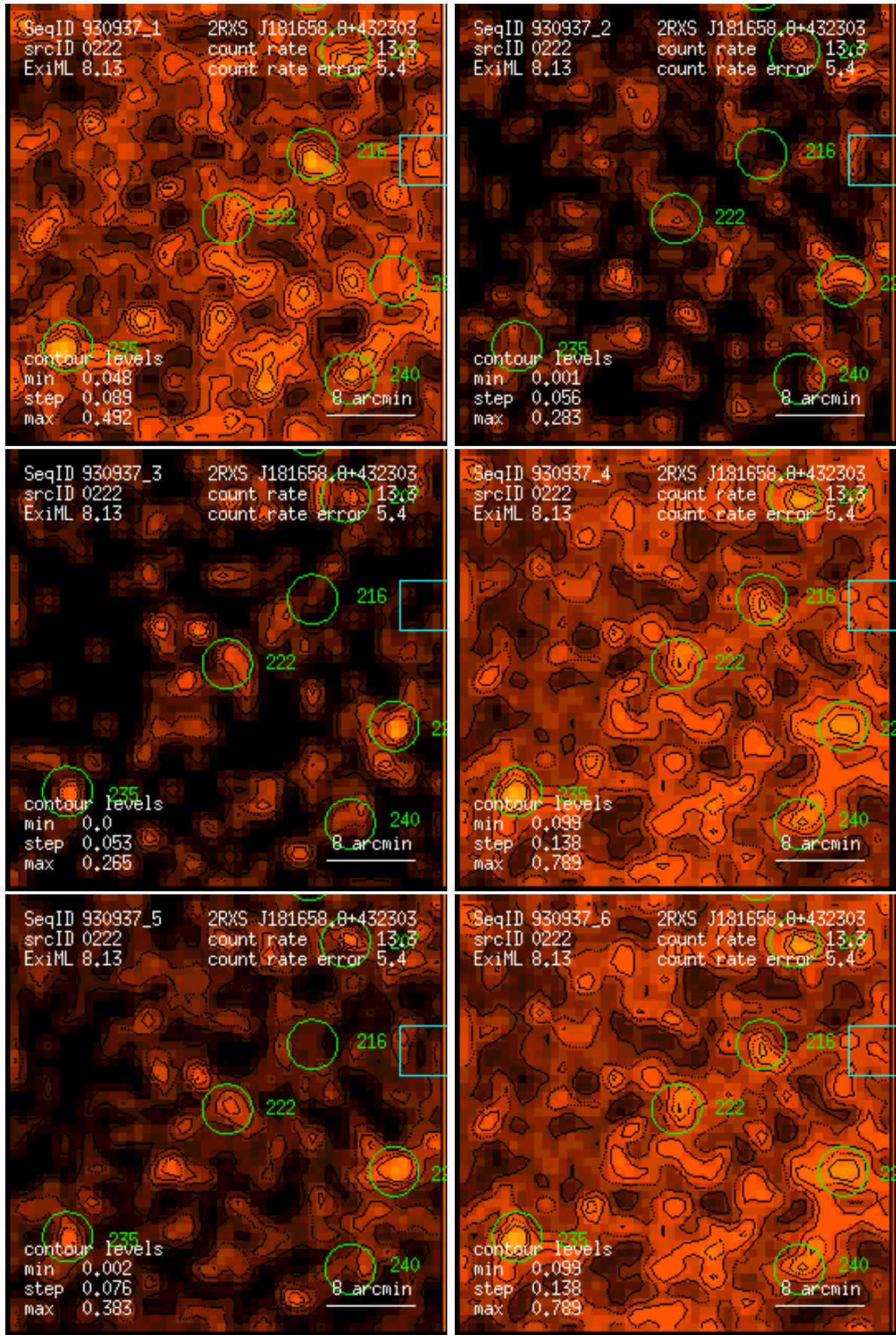
Figure 222: RASS 930937: detection 0222: band rate images, Gaussian filter: (1) PSPC channels 11 – 41, (2) 52 – 90, (3) 91 – 201, (4) 11 – 235, (5) 52 – 201, (6) 11 – 201. Broad band rates in counts/ks. Band rate contour levels in counts/ks/arcmin 2 .
