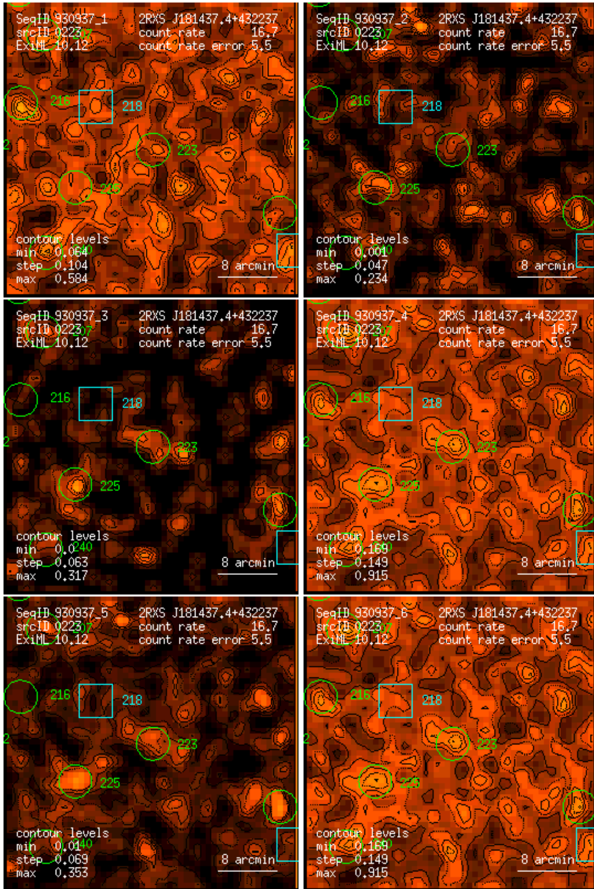
Figure 223: RASS 930937: detection 0223: band rate images, Gaussian filter: (1) PSPC channels 11 – 41, (2) 52 – 90, (3) 91 – 201, (4) 11 – 235, (5) 52 – 201, (6) 11 – 201. Broad band rates in counts/ks. Band rate contour levels in counts/ks/arcmin 2 .
