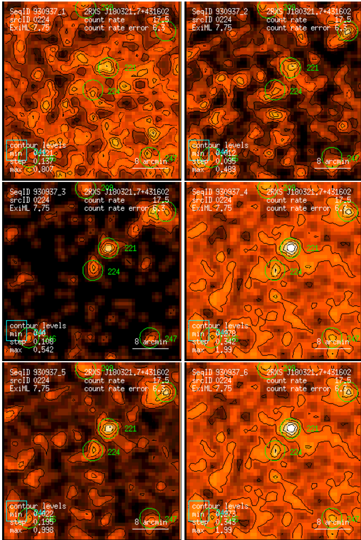
Figure 224: RASS 930937: detection 0224: band rate images, Gaussian filter: (1) PSPC channels 11 – 41, (2) 52 – 90, (3) 91 – 201, (4) 11 – 235, (5) 52 – 201, (6) 11 – 201. Broad band rates in counts/ks. Band rate contour levels in counts/ks/arcmin 2 .
