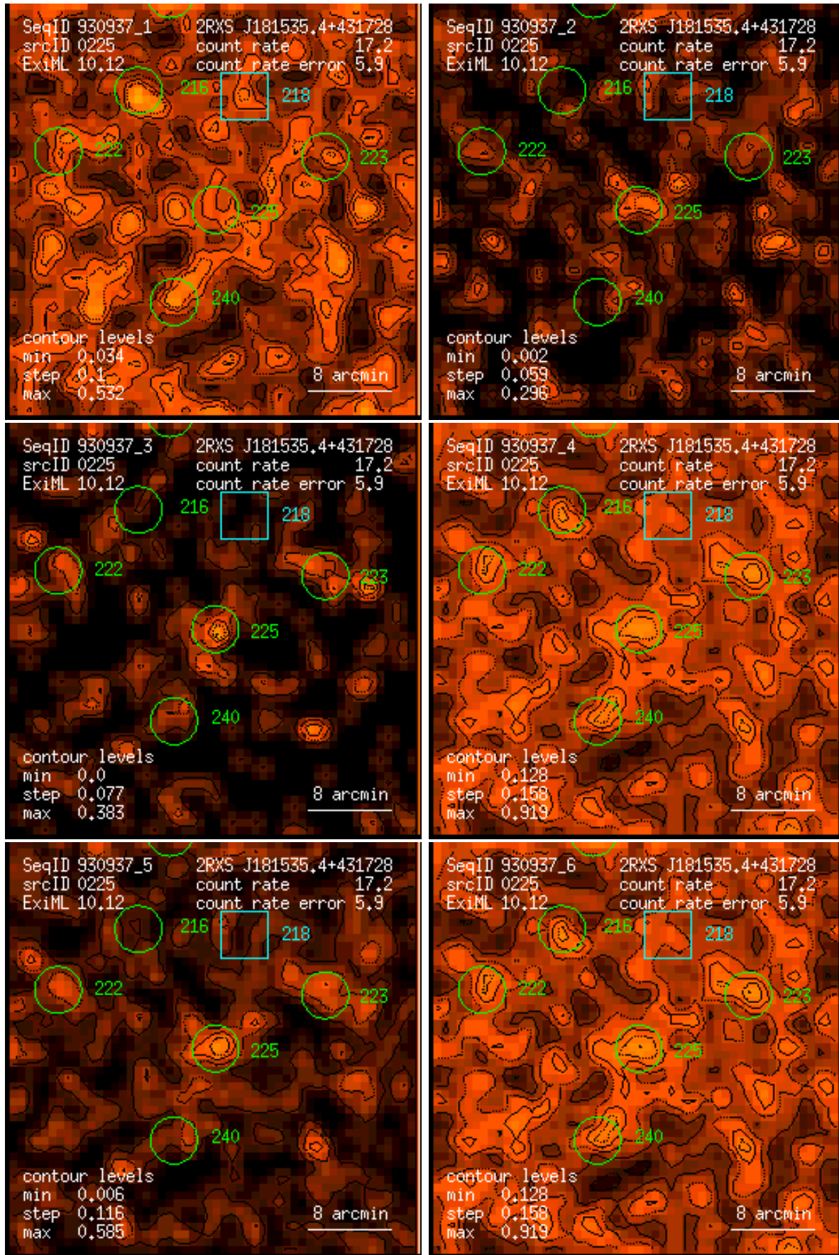
Figure 225: RASS 930937: detection 0225: band rate images, Gaussian filter: (1) PSPC channels 11 – 41, (2) 52 – 90, (3) 91 – 201, (4) 11 – 235, (5) 52 – 201, (6) 11 – 201. Broad band rates in counts/ks. Band rate contour levels in counts/ks/arcmin 2 .
