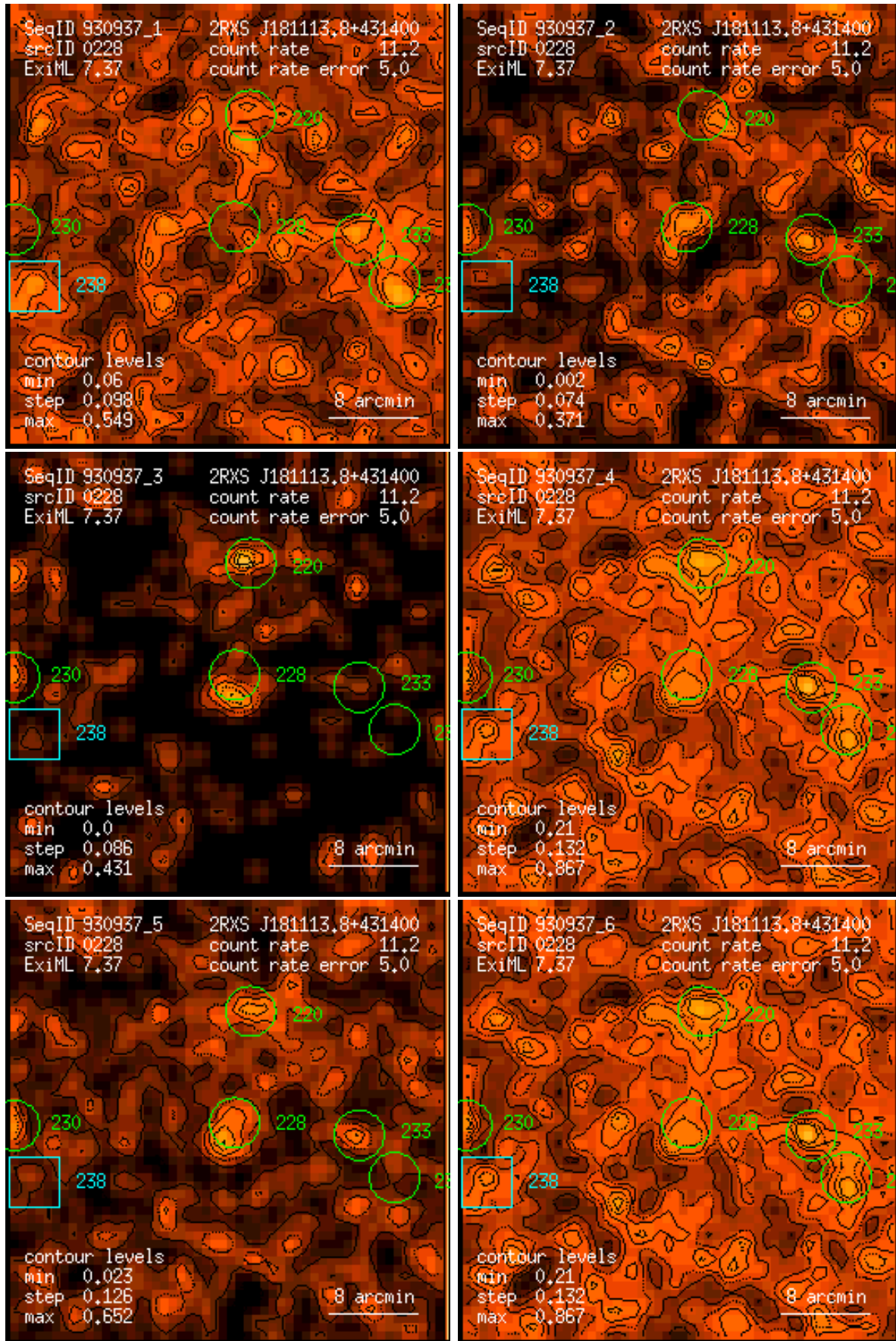
Figure 228: RASS 930937: detection 0228: band rate images, Gaussian filter: (1) PSPC channels 11 – 41, (2) 52 – 90, (3) 91 – 201, (4) 11 – 235, (5) 52 – 201, (6) 11 – 201. Broad band rates in counts/ks. Band rate contour levels in counts/ks/arcmin 2 .
