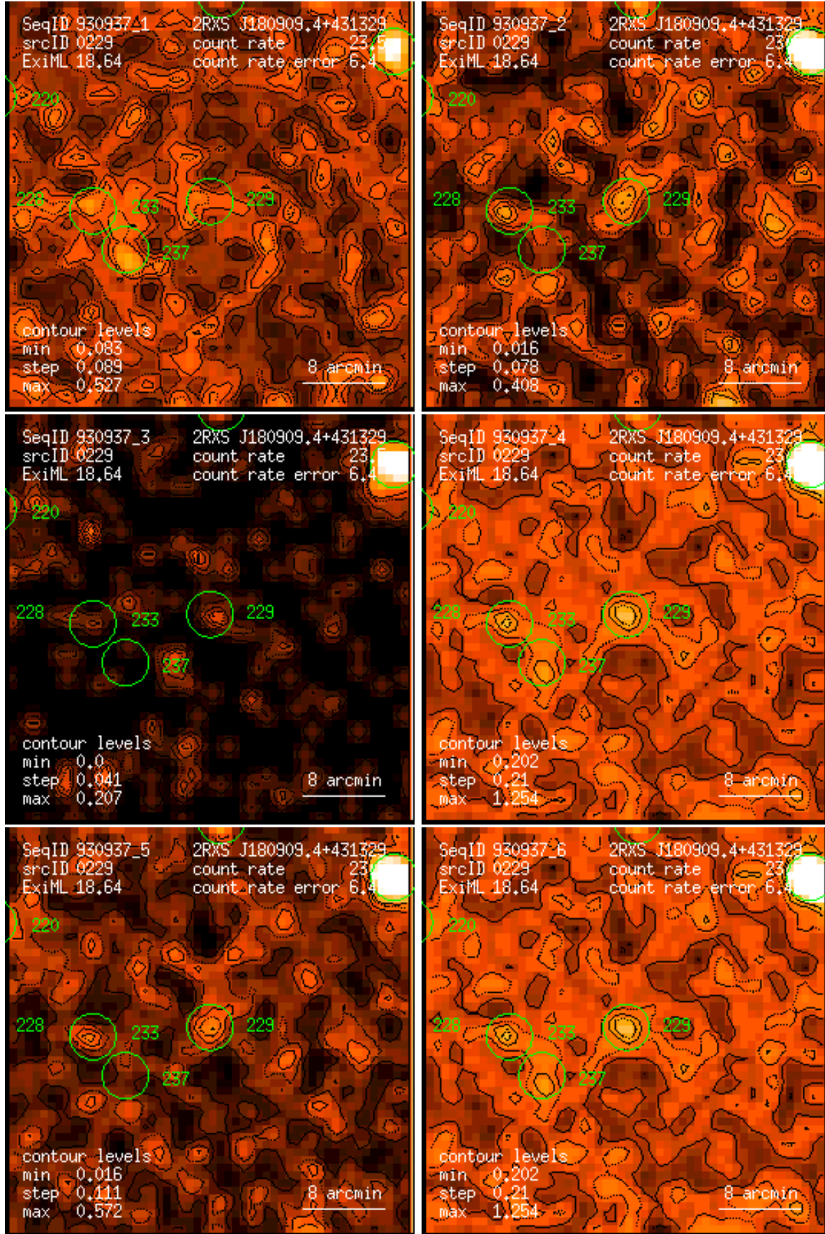
Figure 229: RASS 930937: detection 0229: band rate images, Gaussian filter: (1) PSPC channels 11 – 41, (2) 52 – 90, (3) 91 – 201, (4) 11 – 235, (5) 52 – 201, (6) 11 – 201. Broad band rates in counts/ks. Band rate contour levels in counts/ks/arcmin 2 .
