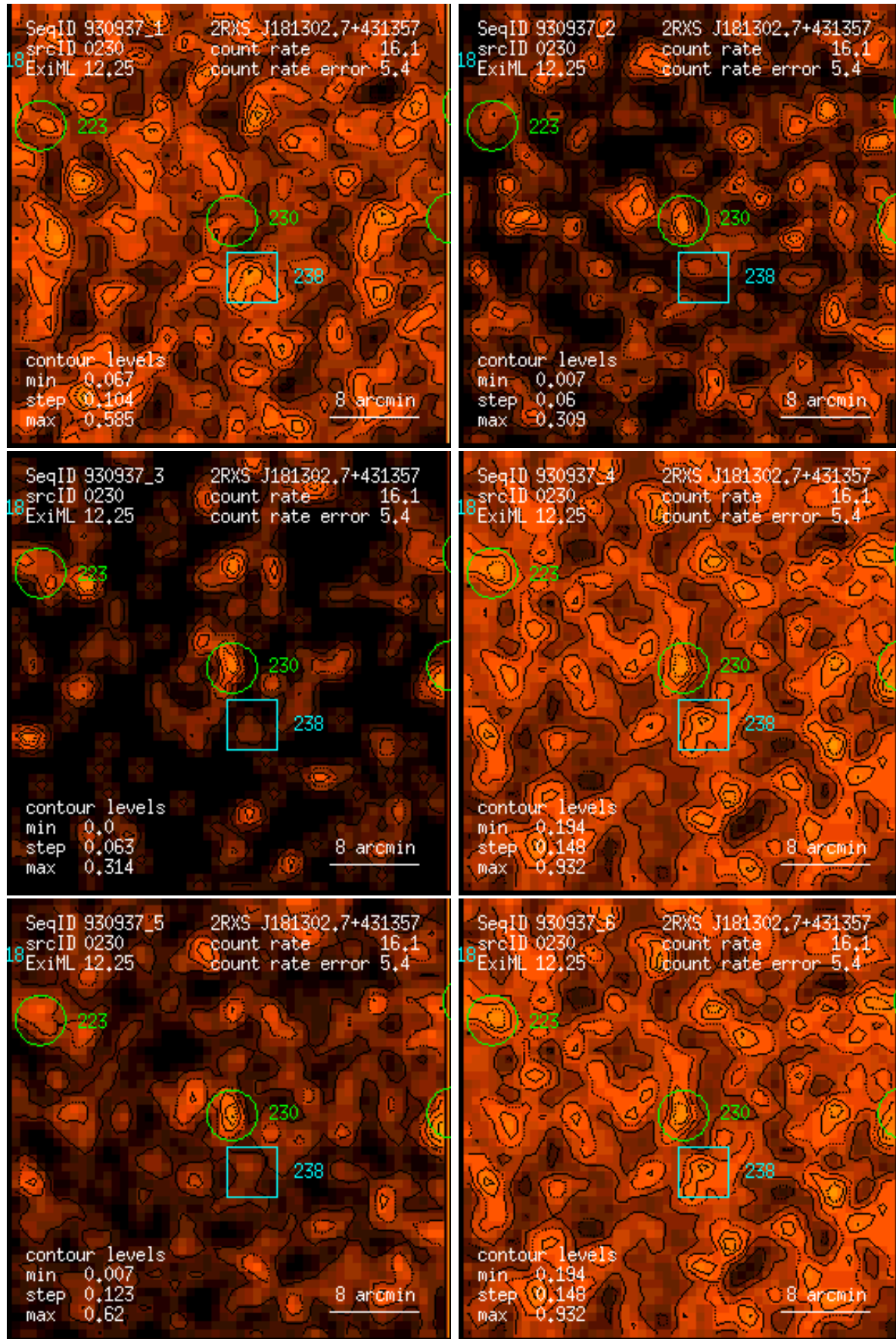
Figure 230: RASS 930937: detection 0230: band rate images, Gaussian filter: (1) PSPC channels 11 – 41, (2) 52 – 90, (3) 91 – 201, (4) 11 – 235, (5) 52 – 201, (6) 11 – 201. Broad band rates in counts/ks. Band rate contour levels in counts/ks/arcmin 2 .
