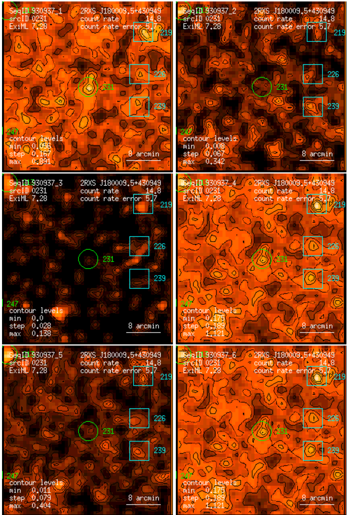
Figure 231: RASS 930937: detection 0231: band rate images, Gaussian filter: (1) PSPC channels 11 – 41, (2) 52 – 90, (3) 91 – 201, (4) 11 – 235, (5) 52 – 201, (6) 11 – 201. Broad band rates in counts/ks. Band rate contour levels in counts/ks/arcmin 2 .
