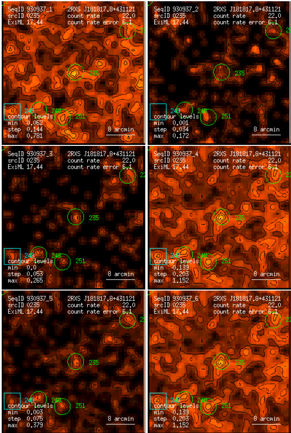
Figure 235: RASS 930937: detection 0235: band rate images, Gaussian filter: (1) PSPC channels 11 – 41, (2) 52 – 90, (3) 91 – 201, (4) 11 – 235, (5) 52 – 201, (6) 11 – 201. Broad band rates in counts/ks. Band rate contour levels in counts/ks/arcmin 2 .
