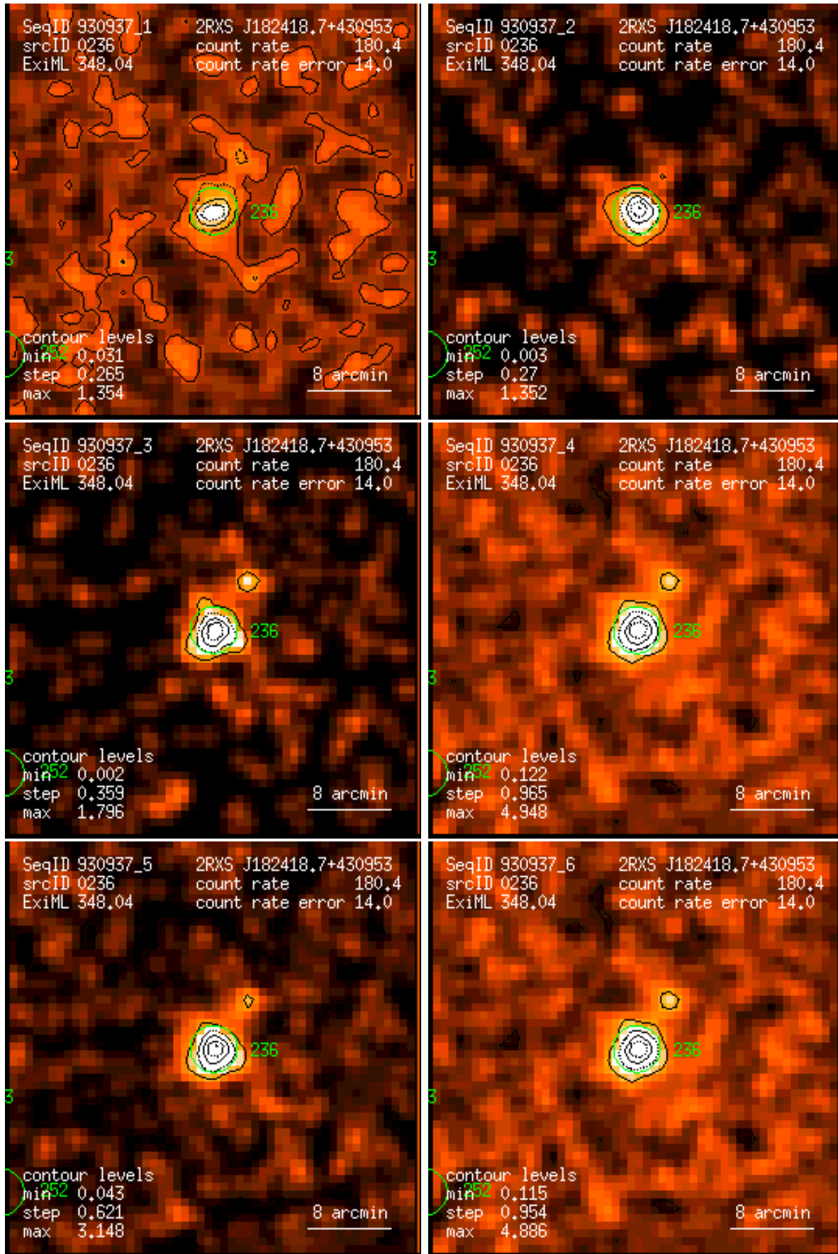
Figure 236: RASS 930937: detection 0236: band rate images, Gaussian filter: (1) PSPC channels 11 – 41, (2) 52 – 90, (3) 91 – 201, (4) 11 – 235, (5) 52 – 201, (6) 11 – 201. Broad band rates in counts/ks. Band rate contour levels in counts/ks/arcmin 2 .
