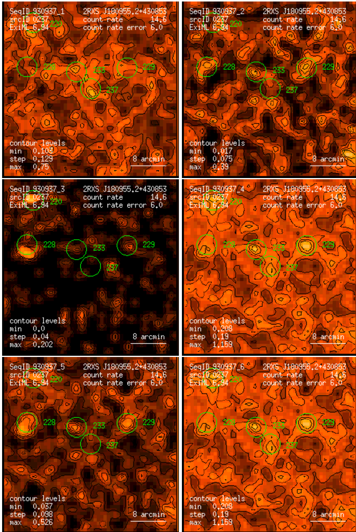
Figure 237: RASS 930937: detection 0237: band rate images, Gaussian filter: (1) PSPC channels 11 – 41, (2) 52 – 90, (3) 91 – 201, (4) 11 – 235, (5) 52 – 201, (6) 11 – 201. Broad band rates in counts/ks. Band rate contour levels in counts/ks/arcmin 2 .
