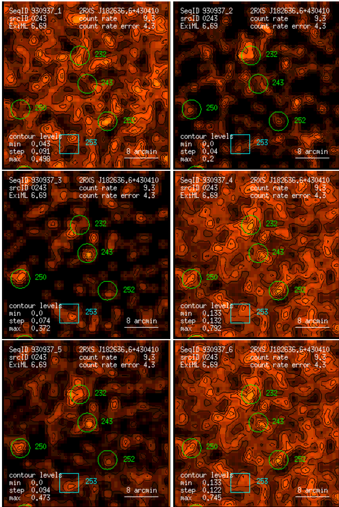
Figure 243: RASS 930937: detection 0243: band rate images, Gaussian filter: (1) PSPC channels 11 – 41, (2) 52 – 90, (3) 91 – 201, (4) 11 – 235, (5) 52 – 201, (6) 11 – 201. Broad band rates in counts/ks. Band rate contour levels in counts/ks/arcmin 2 .
