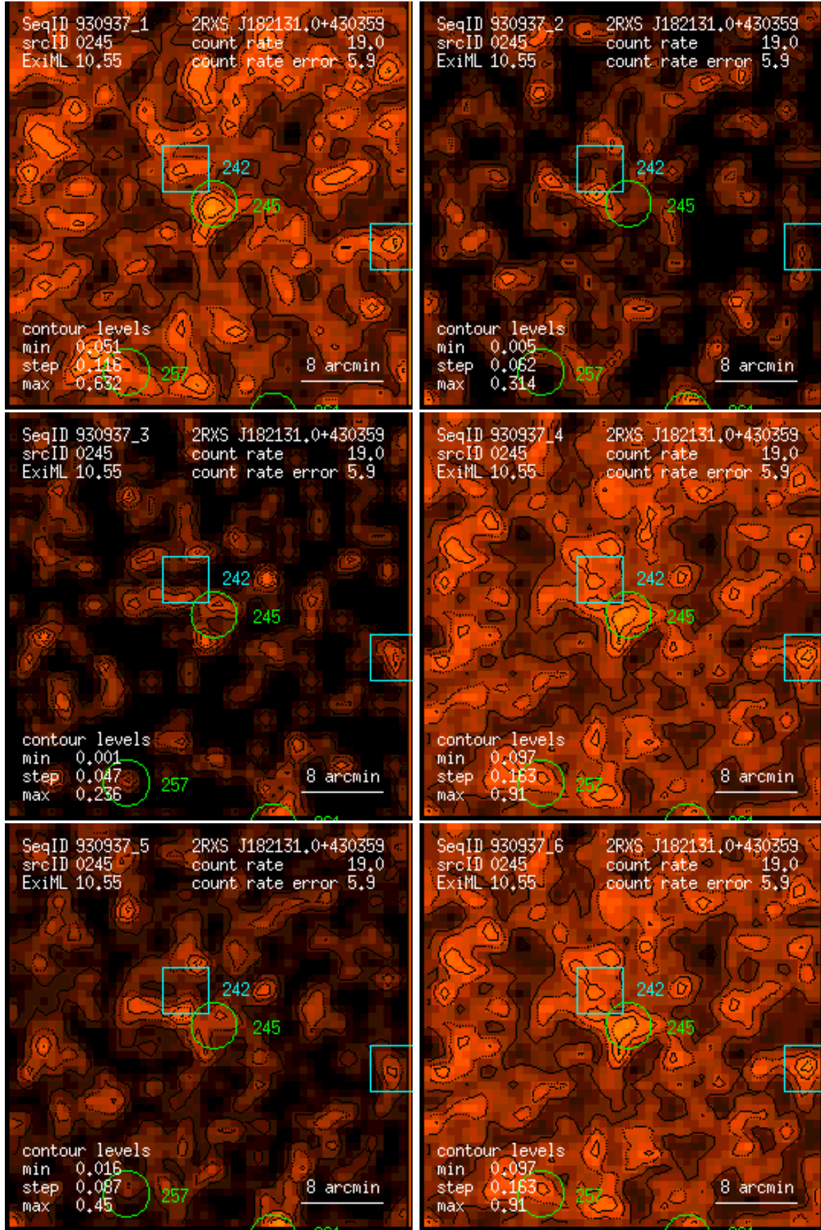
Figure 245: RASS 930937: detection 0245: band rate images, Gaussian filter: (1) PSPC channels 11 – 41, (2) 52 – 90, (3) 91 – 201, (4) 11 – 235, (5) 52 – 201, (6) 11 – 201. Broad band rates in counts/ks. Band rate contour levels in counts/ks/arcmin 2 .
