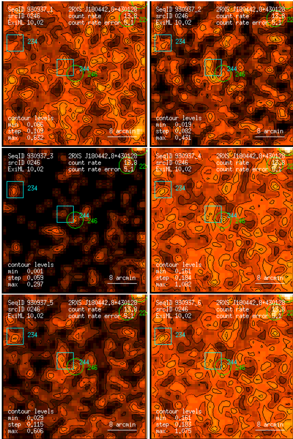
Figure 246: RASS 930937: detection 0246: band rate images, Gaussian filter: (1) PSPC channels 11 – 41, (2) 52 – 90, (3) 91 – 201, (4) 11 – 235, (5) 52 – 201, (6) 11 – 201. Broad band rates in counts/ks. Band rate contour levels in counts/ks/arcmin 2 .
