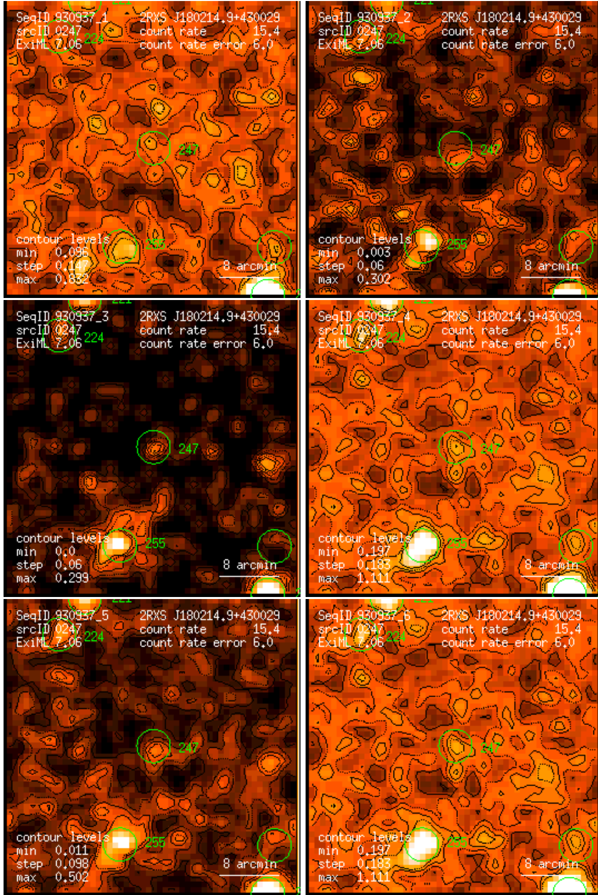
Figure 247: RASS 930937: detection 0247: band rate images, Gaussian filter: (1) PSPC channels 11 – 41, (2) 52 – 90, (3) 91 – 201, (4) 11 – 235, (5) 52 – 201, (6) 11 – 201. Broad band rates in counts/ks. Band rate contour levels in counts/ks/arcmin 2 .
