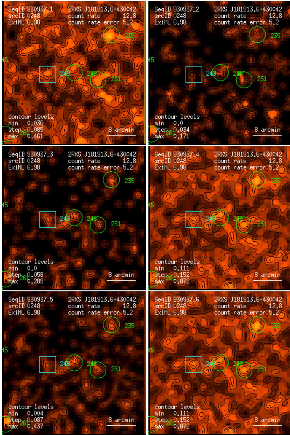
Figure 248: RASS 930937: detection 0248: band rate images, Gaussian filter: (1) PSPC channels 11 – 41, (2) 52 – 90, (3) 91 – 201, (4) 11 – 235, (5) 52 – 201, (6) 11 – 201. Broad band rates in counts/ks. Band rate contour levels in counts/ks/arcmin 2 .
