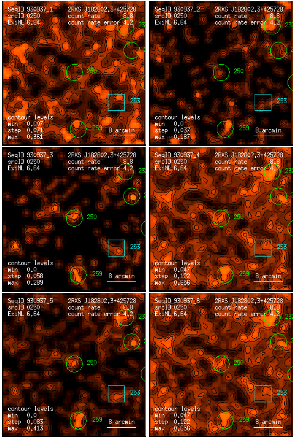
Figure 250: RASS 930937: detection 0250: band rate images, Gaussian filter: (1) PSPC channels 11 – 41, (2) 52 – 90, (3) 91 – 201, (4) 11 – 235, (5) 52 – 201, (6) 11 – 201. Broad band rates in counts/ks. Band rate contour levels in counts/ks/arcmin 2 .
