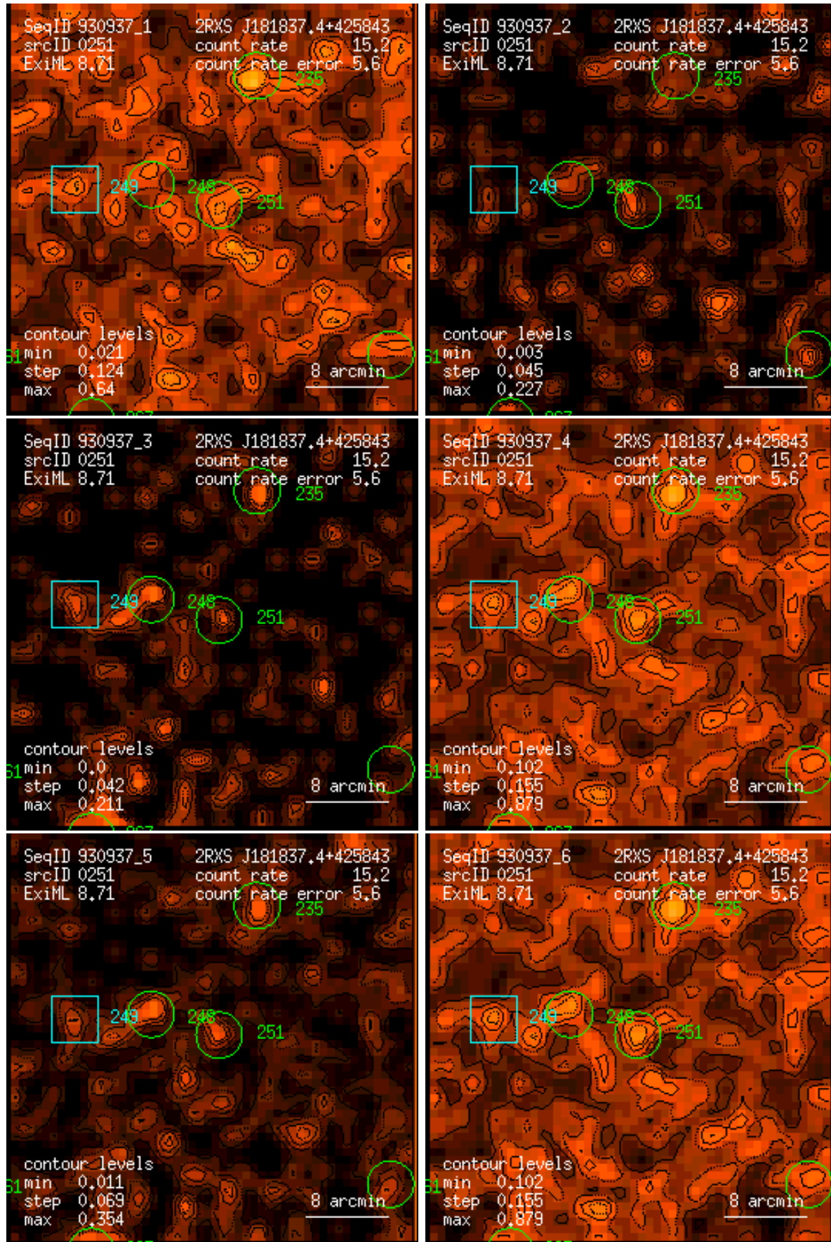
Figure 251: RASS 930937: detection 0251: band rate images, Gaussian filter: (1) PSPC channels 11 – 41, (2) 52 – 90, (3) 91 – 201, (4) 11 – 235, (5) 52 – 201, (6) 11 – 201. Broad band rates in counts/ks. Band rate contour levels in counts/ks/arcmin 2 .
