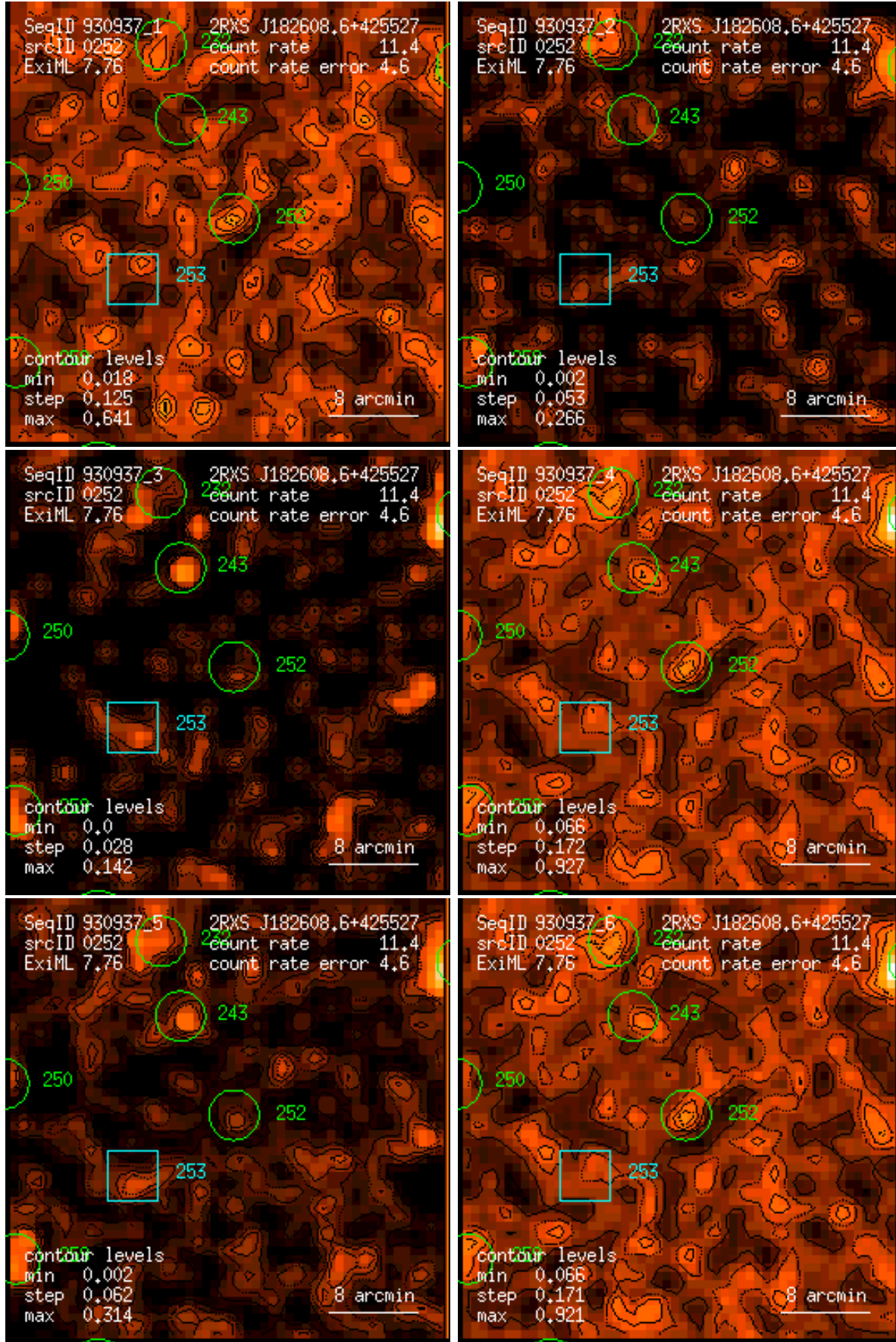
Figure 252: RASS 930937: detection 0252: band rate images, Gaussian filter: (1) PSPC channels 11 – 41, (2) 52 – 90, (3) 91 – 201, (4) 11 – 235, (5) 52 – 201, (6) 11 – 201. Broad band rates in counts/ks. Band rate contour levels in counts/ks/arcmin 2 .
