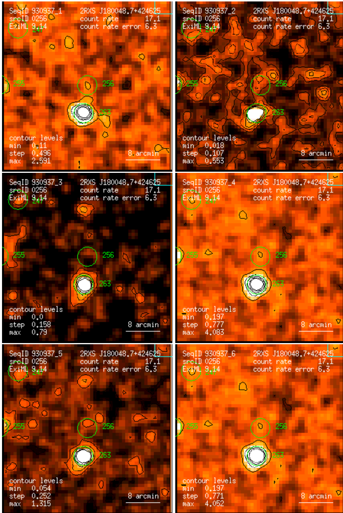
Figure 256: RASS 930937: detection 0256: band rate images, Gaussian filter: (1) PSPC channels 11 – 41, (2) 52 – 90, (3) 91 – 201, (4) 11 – 235, (5) 52 – 201, (6) 11 – 201. Broad band rates in counts/ks. Band rate contour levels in counts/ks/arcmin 2 .
