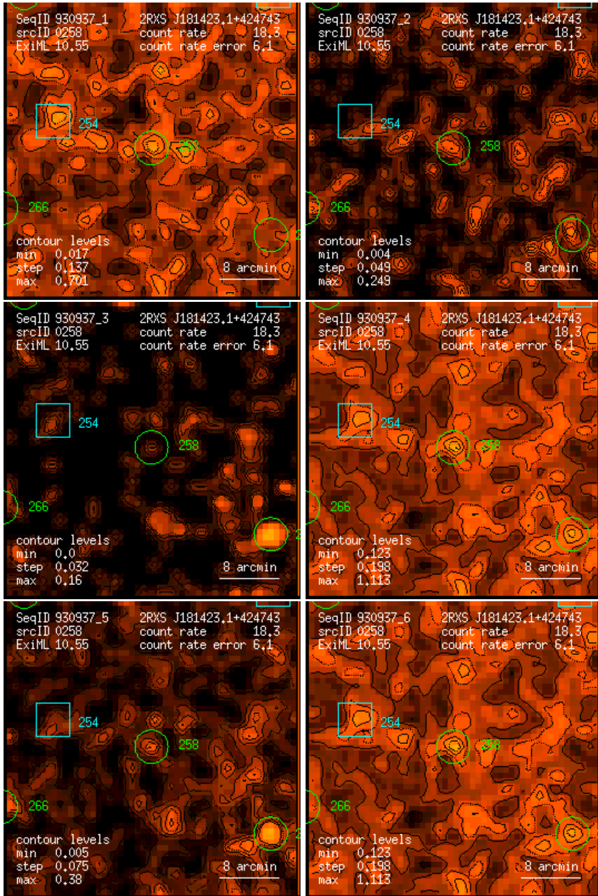
Figure 258: RASS 930937: detection 0258: band rate images, Gaussian filter: (1) PSPC channels 11 – 41, (2) 52 – 90, (3) 91 – 201, (4) 11 – 235, (5) 52 – 201, (6) 11 – 201. Broad band rates in counts/ks. Band rate contour levels in counts/ks/arcmin 2 .
