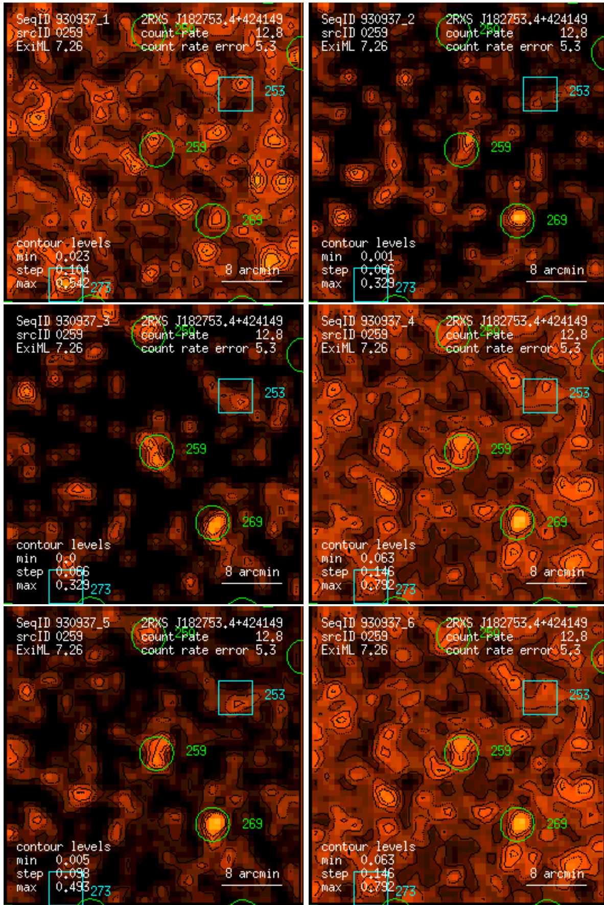
Figure 259: RASS 930937: detection 0259: band rate images, Gaussian filter: (1) PSPC channels 11 – 41, (2) 52 – 90, (3) 91 – 201, (4) 11 – 235, (5) 52 – 201, (6) 11 – 201. Broad band rates in counts/ks. Band rate contour levels in counts/ks/arcmin 2 .
