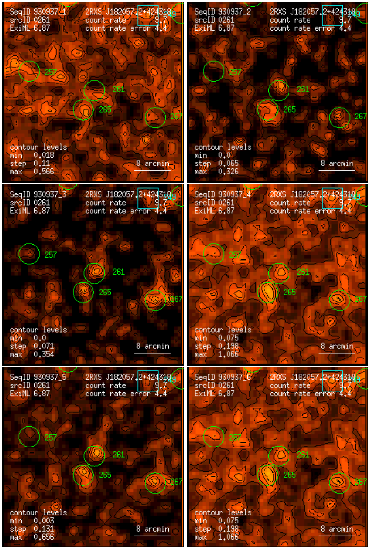
Figure 261: RASS 930937: detection 0261: band rate images, Gaussian filter: (1) PSPC channels 11 – 41, (2) 52 – 90, (3) 91 – 201, (4) 11 – 235, (5) 52 – 201, (6) 11 – 201. Broad band rates in counts/ks. Band rate contour levels in counts/ks/arcmin 2 .
