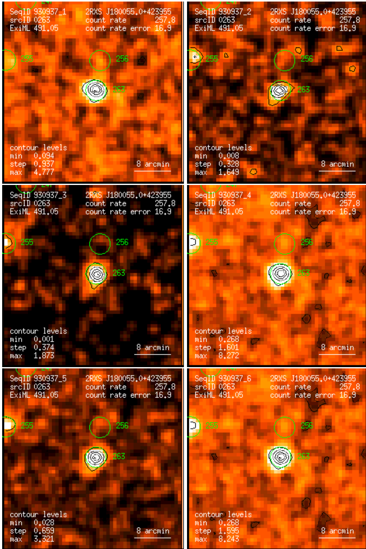
Figure 263: RASS 930937: detection 0263: band rate images, Gaussian filter: (1) PSPC channels 11 – 41, (2) 52 – 90, (3) 91 – 201, (4) 11 – 235, (5) 52 – 201, (6) 11 – 201. Broad band rates in counts/ks. Band rate contour levels in counts/ks/arcmin 2 .
