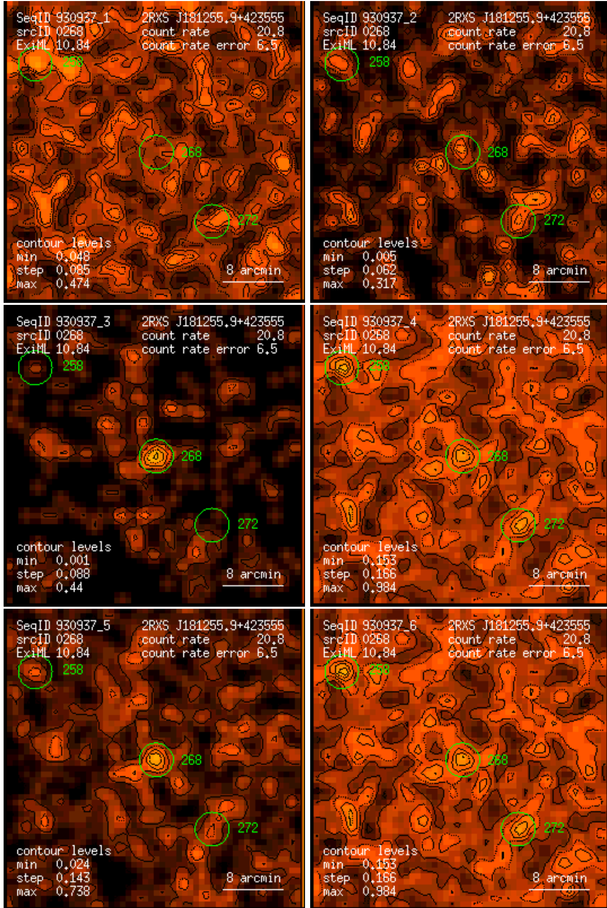
Figure 268: RASS 930937: detection 0268: band rate images, Gaussian filter: (1) PSPC channels 11 – 41, (2) 52 – 90, (3) 91 – 201, (4) 11 – 235, (5) 52 – 201, (6) 11 – 201. Broad band rates in counts/ks. Band rate contour levels in counts/ks/arcmin 2 .
