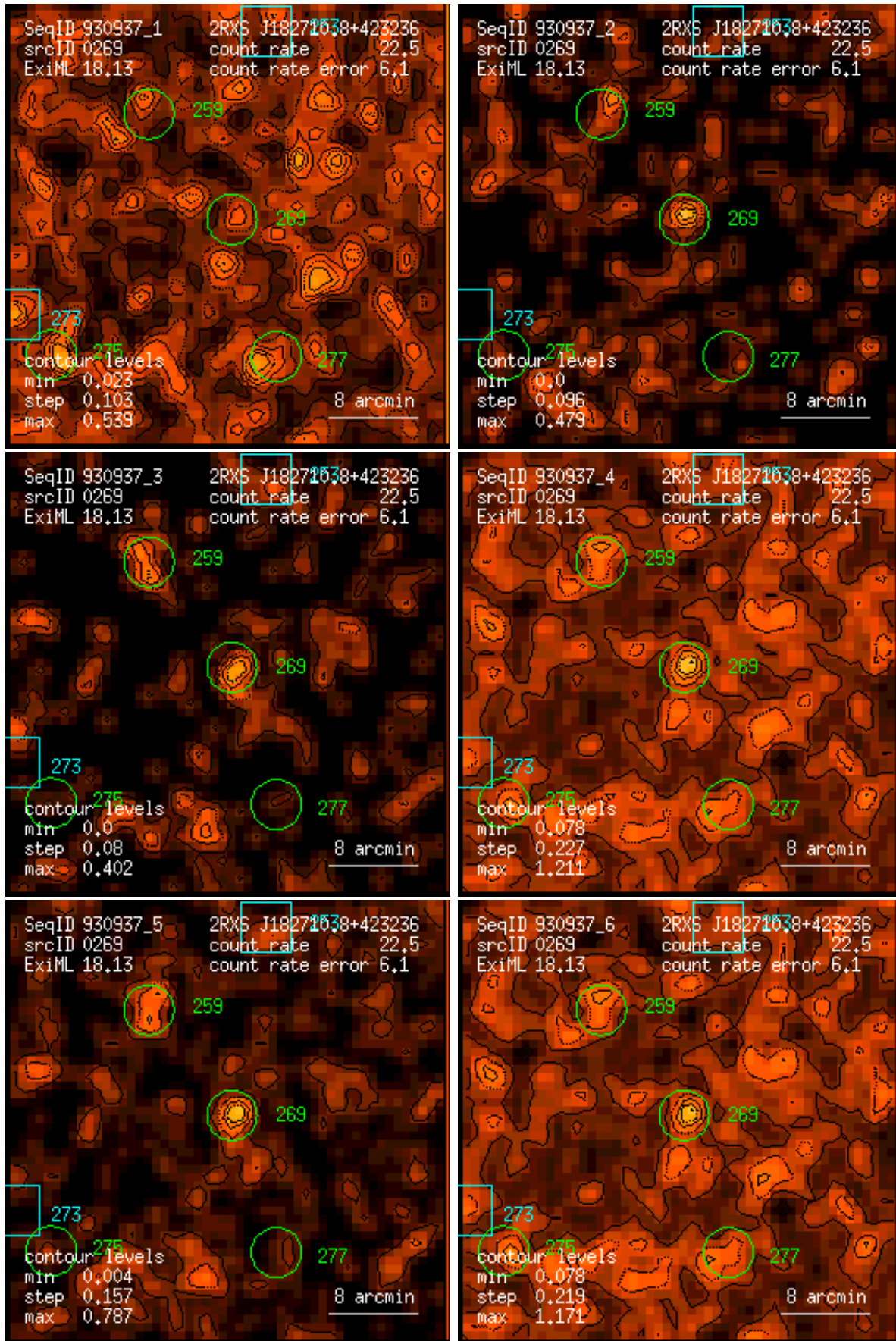
Figure 269: RASS 930937: detection 0269: band rate images, Gaussian filter: (1) PSPC channels 11 – 41, (2) 52 – 90, (3) 91 – 201, (4) 11 – 235, (5) 52 – 201, (6) 11 – 201. Broad band rates in counts/ks. Band rate contour levels in counts/ks/arcmin 2 .
