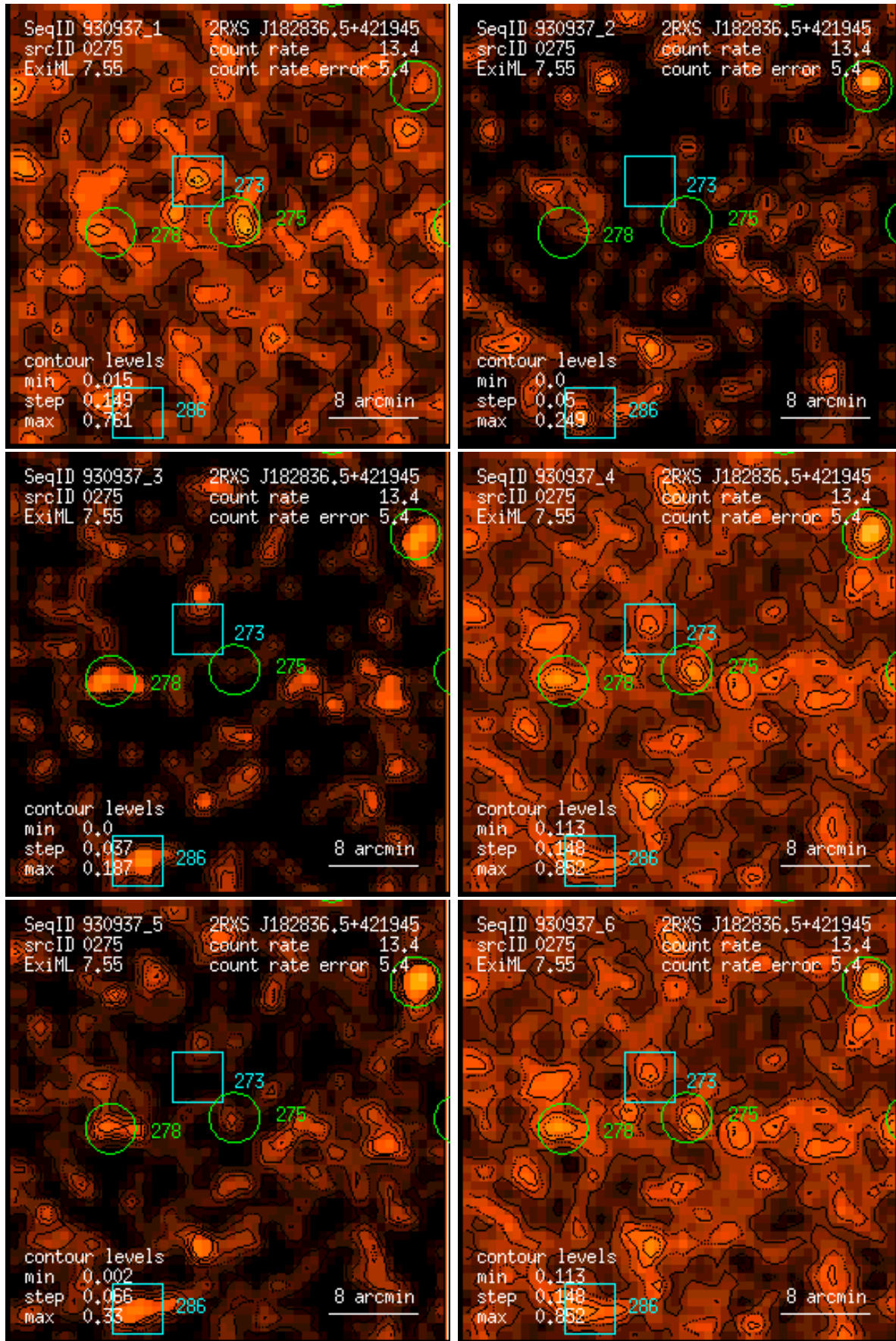
Figure 275: RASS 930937: detection 0275: band rate images, Gaussian filter: (1) PSPC channels 11 – 41, (2) 52 – 90, (3) 91 – 201, (4) 11 – 235, (5) 52 – 201, (6) 11 – 201. Broad band rates in counts/ks. Band rate contour levels in counts/ks/arcmin 2 .
