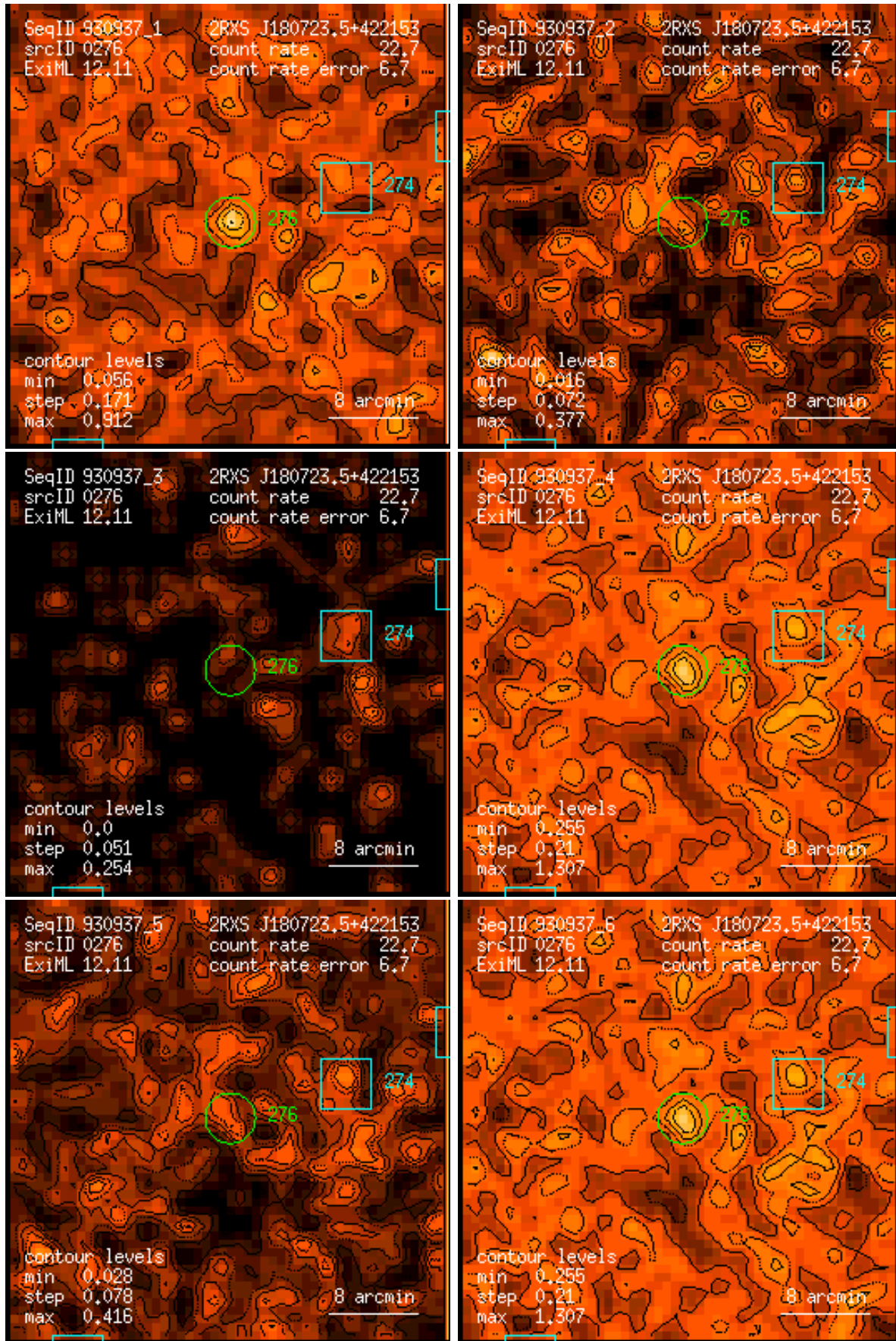
Figure 276: RASS 930937: detection 0276: band rate images, Gaussian filter: (1) PSPC channels 11 – 41, (2) 52 – 90, (3) 91 – 201, (4) 11 – 235, (5) 52 – 201, (6) 11 – 201. Broad band rates in counts/ks. Band rate contour levels in counts/ks/arcmin 2 .
