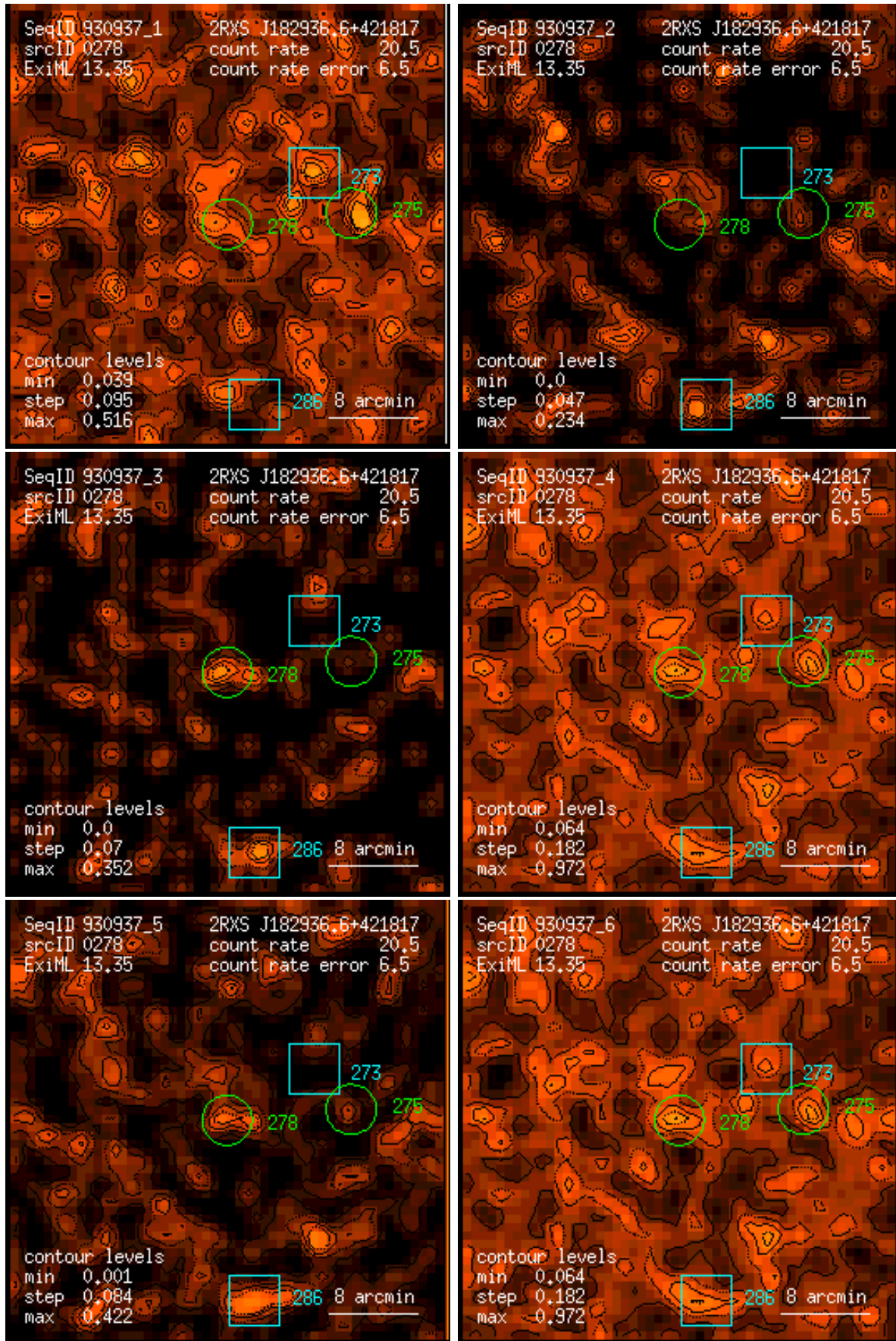
Figure 278: RASS 930937: detection 0278: band rate images, Gaussian filter: (1) PSPC channels 11 – 41, (2) 52 – 90, (3) 91 – 201, (4) 11 – 235, (5) 52 – 201, (6) 11 – 201. Broad band rates in counts/ks. Band rate contour levels in counts/ks/arcmin 2 .
