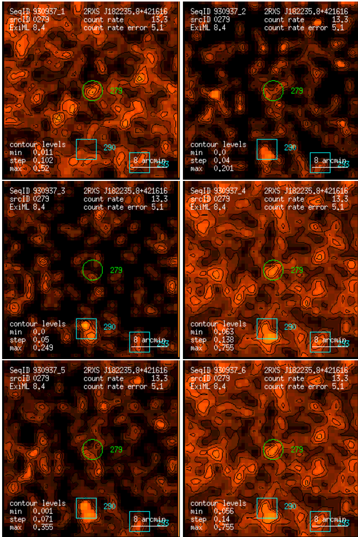
Figure 279: RASS 930937: detection 0279: band rate images, Gaussian filter: (1) PSPC channels 11 – 41, (2) 52 – 90, (3) 91 – 201, (4) 11 – 235, (5) 52 – 201, (6) 11 – 201. Broad band rates in counts/ks. Band rate contour levels in counts/ks/arcmin 2 .
