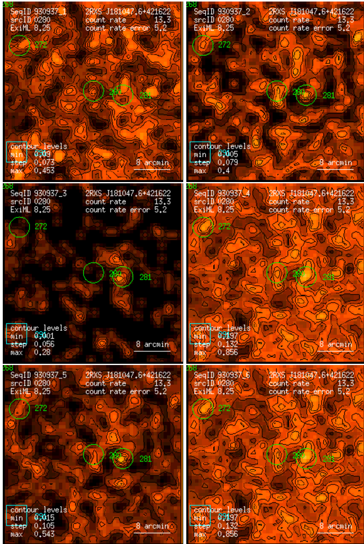
Figure 280: RASS 930937: detection 0280: band rate images, Gaussian filter: (1) PSPC channels 11 – 41, (2) 52 – 90, (3) 91 – 201, (4) 11 – 235, (5) 52 – 201, (6) 11 – 201. Broad band rates in counts/ks. Band rate contour levels in counts/ks/arcmin 2 .
