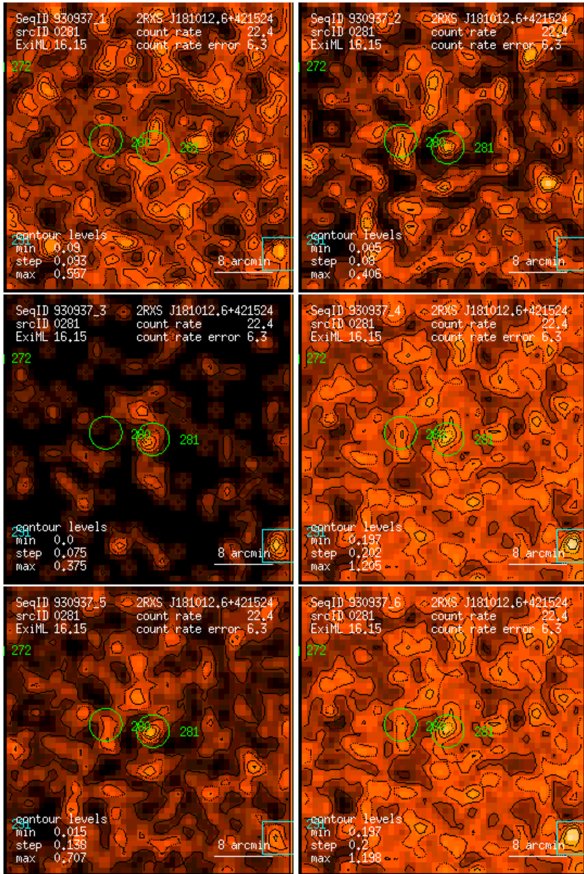
Figure 281: RASS 930937: detection 0281: band rate images, Gaussian filter: (1) PSPC channels 11 – 41, (2) 52 – 90, (3) 91 – 201, (4) 11 – 235, (5) 52 – 201, (6) 11 – 201. Broad band rates in counts/ks. Band rate contour levels in counts/ks/arcmin 2 .
