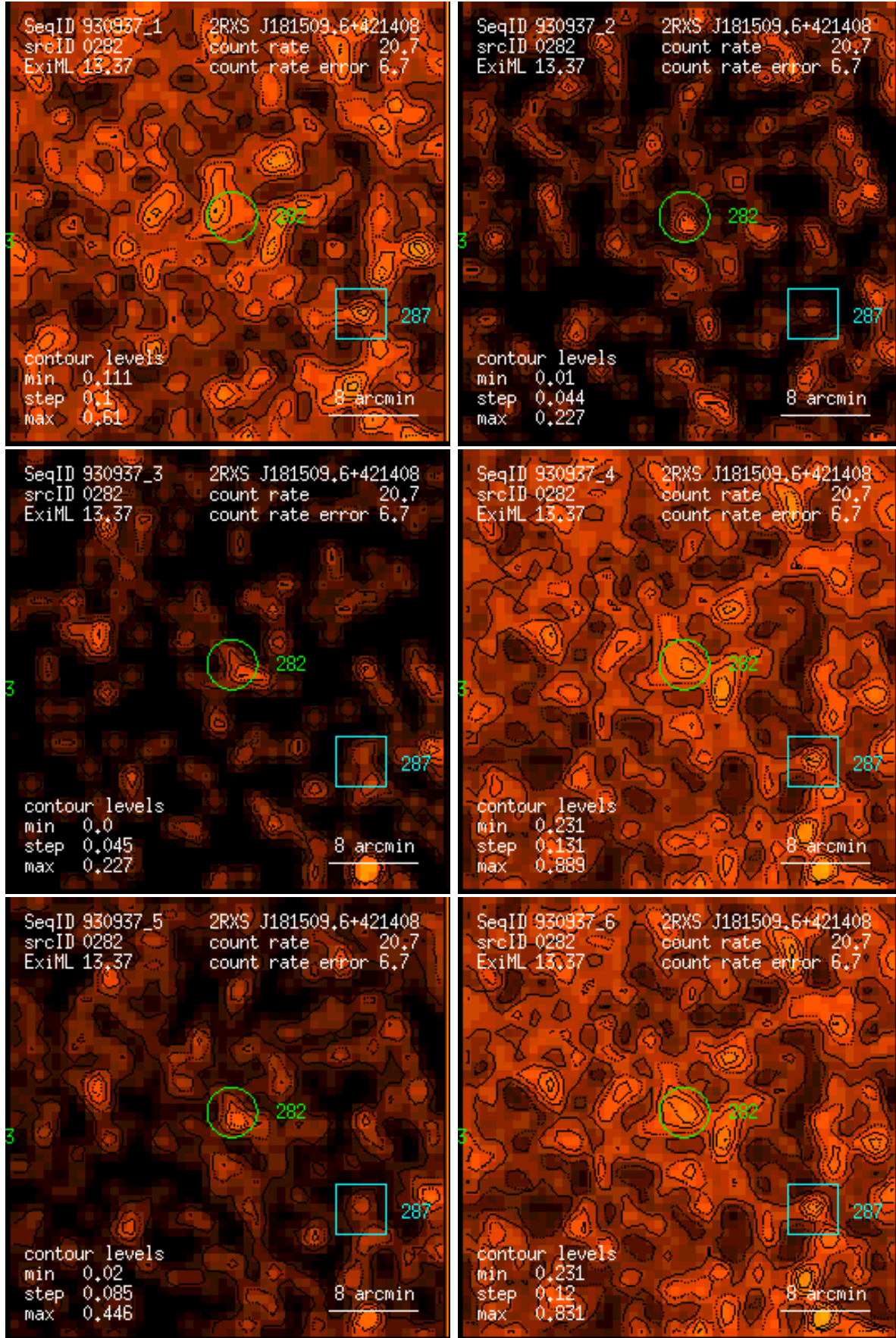
Figure 282: RASS 930937: detection 0282: band rate images, Gaussian filter: (1) PSPC channels 11 – 41, (2) 52 – 90, (3) 91 – 201, (4) 11 – 235, (5) 52 – 201, (6) 11 – 201. Broad band rates in counts/ks. Band rate contour levels in counts/ks/arcmin 2 .
