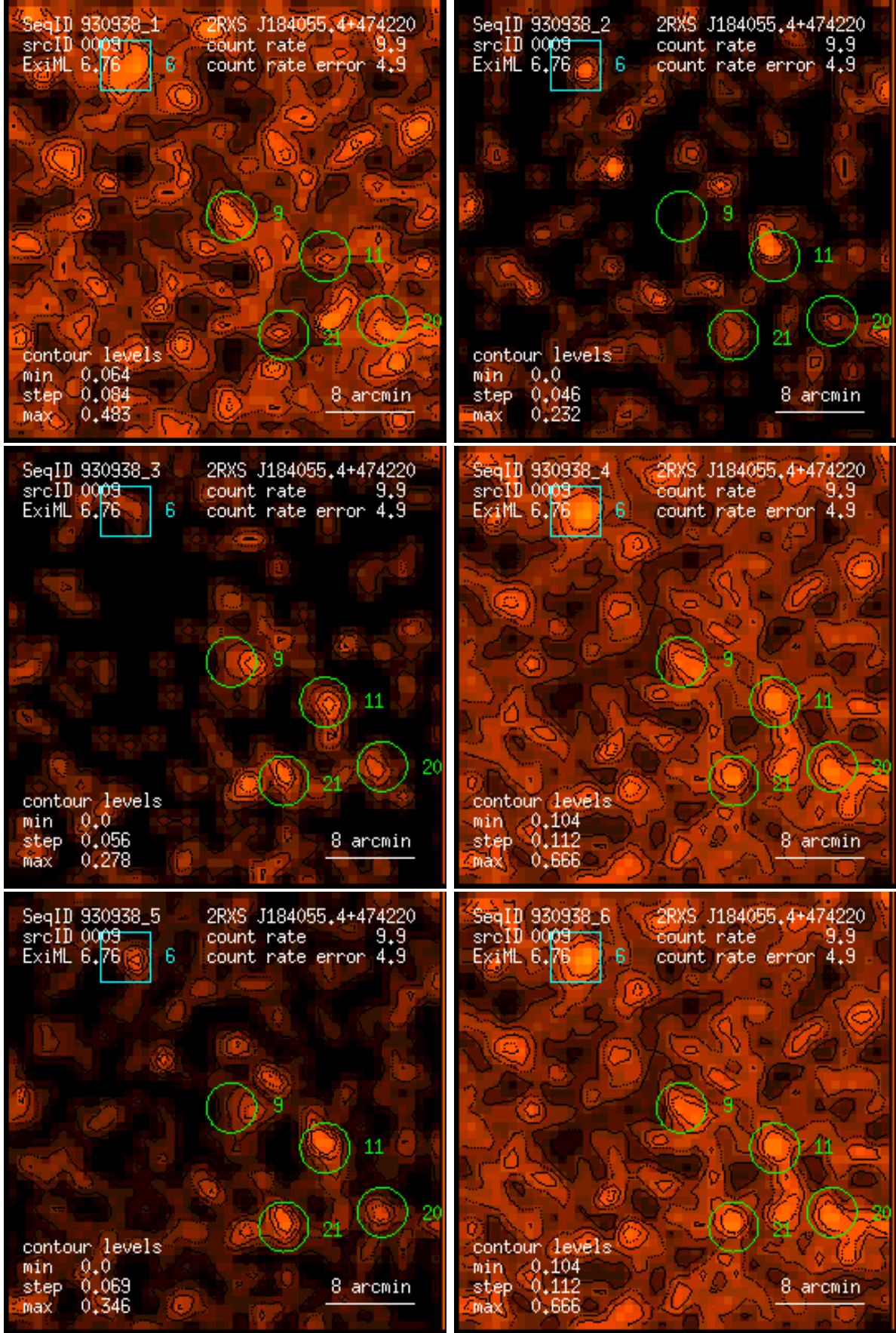
Figure 9: RASS 930938: detection 0009: band rate images, Gaussian filter: (1) PSPC channels 11 – 41, (2) 52 – 90, (3) 91 – 201, (4) 11 – 235, (5) 52 – 201, (6) 11 – 201. Broad band rates in counts/ks. Band rate contour levels in counts/ks/arcmin 2 .
