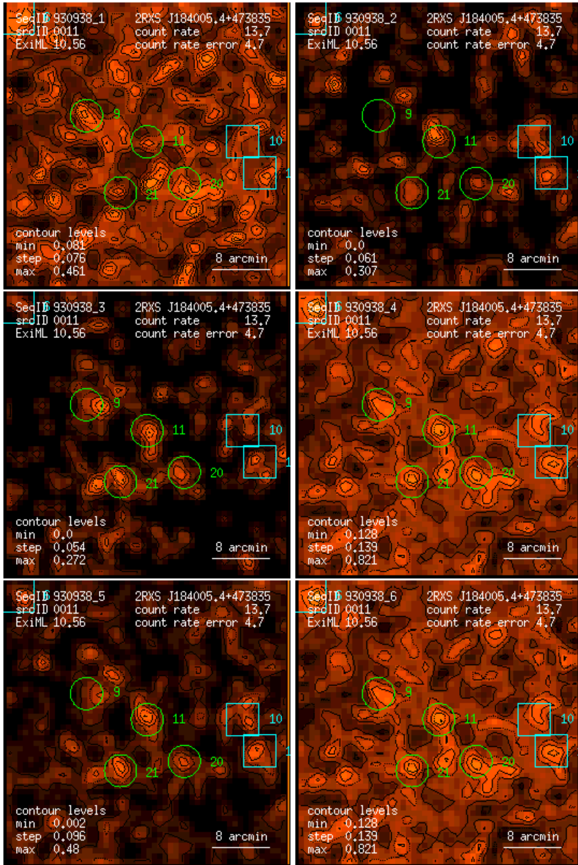
Figure 11: RASS 930938: detection 0011: band rate images, Gaussian filter: (1) PSPC channels 11 – 41, (2) 52 – 90, (3) 91 – 201, (4) 11 – 235, (5) 52 – 201, (6) 11 – 201. Broad band rates in counts/ks. Band rate contour levels in counts/ks/arcmin 2 .
