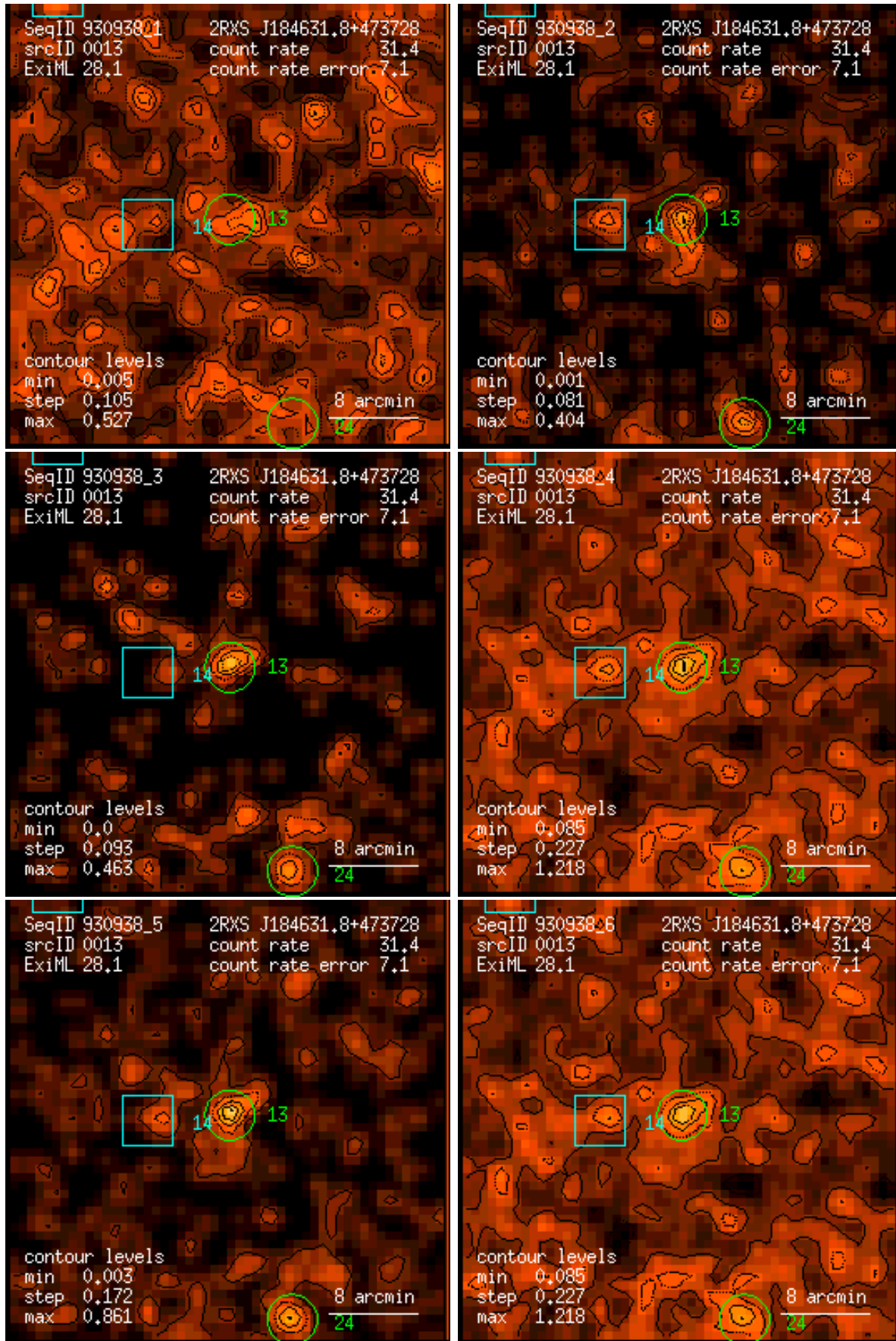
Figure 13: RASS 930938: detection 0013: band rate images, Gaussian filter: (1) PSPC channels 11 – 41, (2) 52 – 90, (3) 91 – 201, (4) 11 – 235, (5) 52 – 201, (6) 11 – 201. Broad band rates in counts/ks. Band rate contour levels in counts/ks/arcmin 2 .
