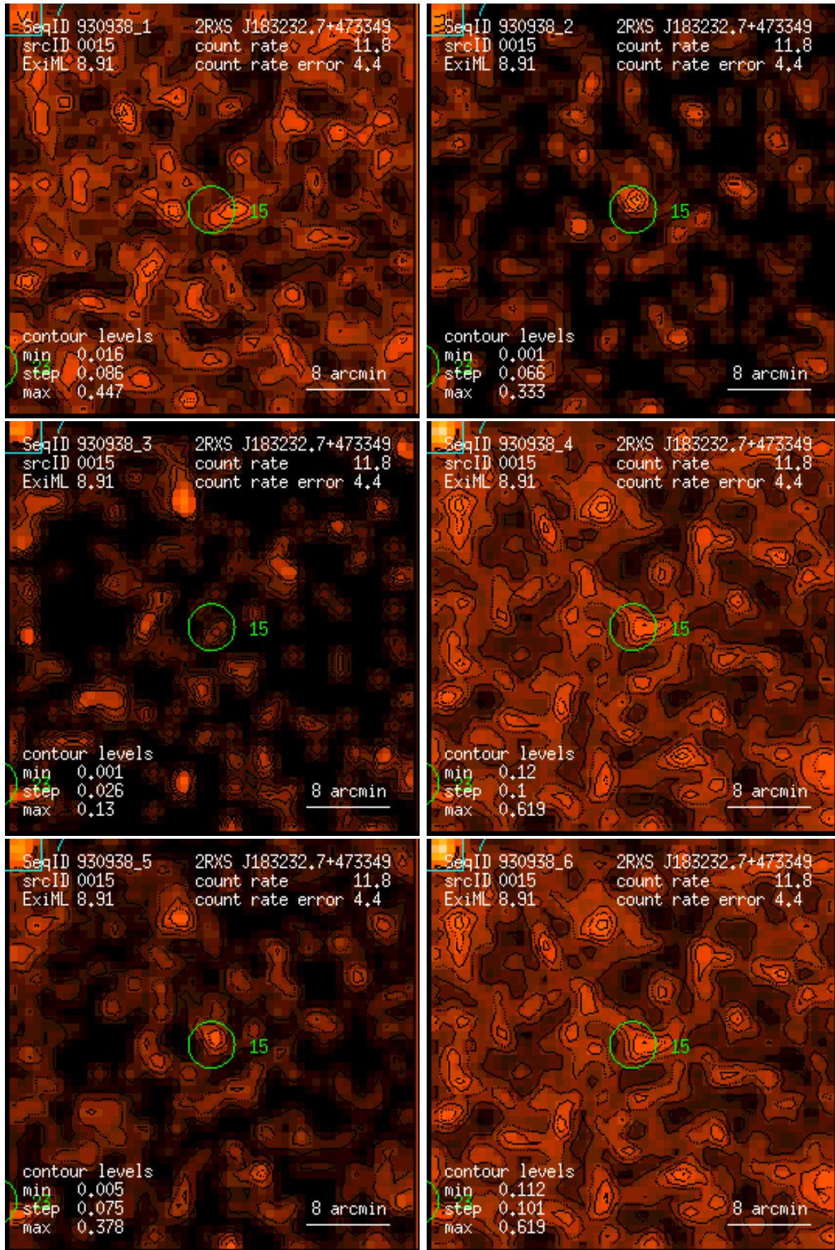
Figure 15: RASS 930938: detection 0015: band rate images, Gaussian filter: (1) PSPC channels 11 – 41, (2) 52 – 90, (3) 91 – 201, (4) 11 – 235, (5) 52 – 201, (6) 11 – 201. Broad band rates in counts/ks. Band rate contour levels in counts/ks/arcmin 2 .
