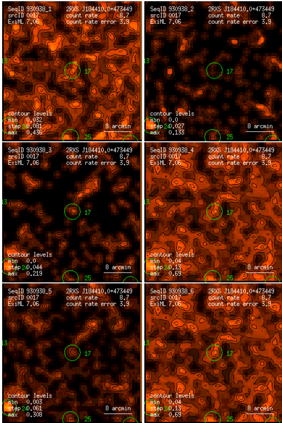
Figure 17: RASS 930938: detection 0017: band rate images, Gaussian filter: (1) PSPC channels 11 – 41, (2) 52 – 90, (3) 91 – 201, (4) 11 – 235, (5) 52 – 201, (6) 11 – 201. Broad band rates in counts/ks. Band rate contour levels in counts/ks/arcmin 2 .
