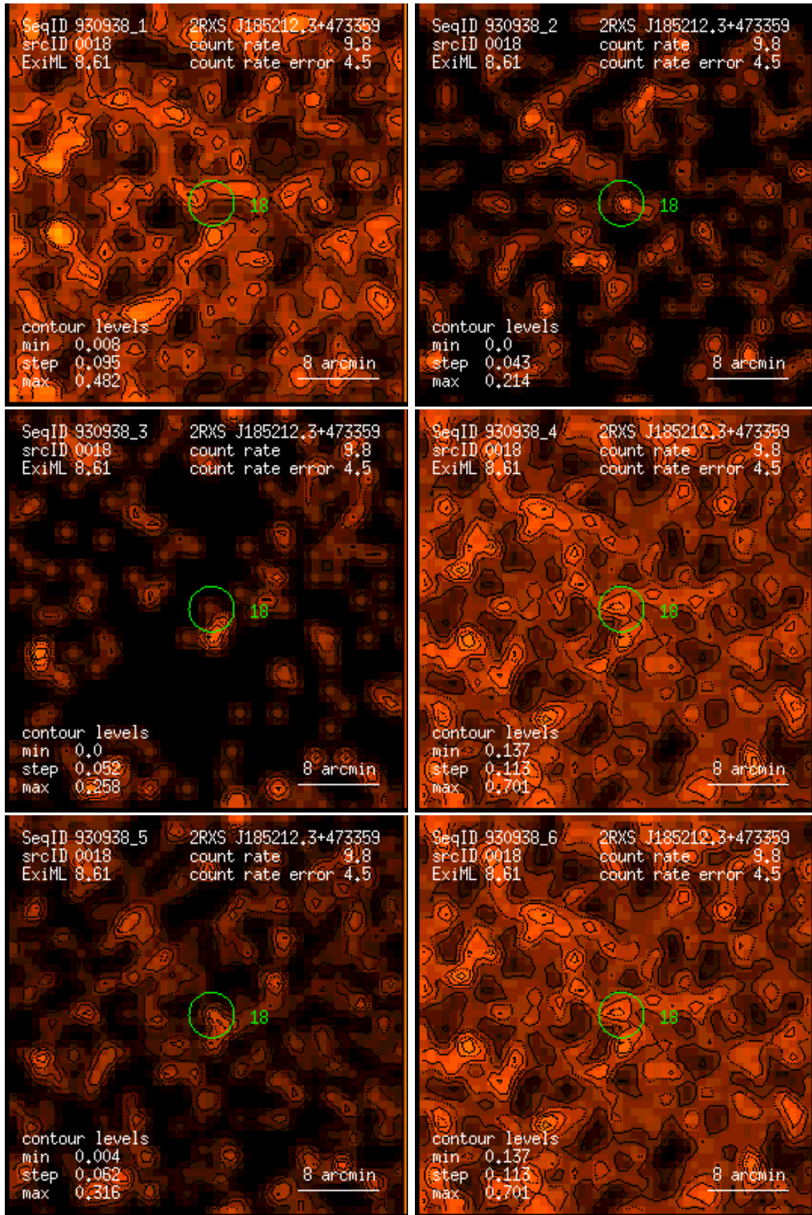
Figure 18: RASS 930938: detection 0018: band rate images, Gaussian filter: (1) PSPC channels 11 – 41, (2) 52 – 90, (3) 91 – 201, (4) 11 – 235, (5) 52 – 201, (6) 11 – 201. Broad band rates in counts/ks. Band rate contour levels in counts/ks/arcmin 2 .
