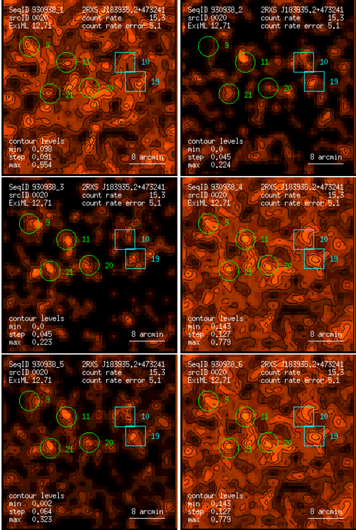
Figure 20: RASS 930938: detection 0020: band rate images, Gaussian filter: (1) PSPC channels 11 – 41, (2) 52 – 90, (3) 91 – 201, (4) 11 – 235, (5) 52 – 201, (6) 11 – 201. Broad band rates in counts/ks. Band rate contour levels in counts/ks/arcmin 2 .
