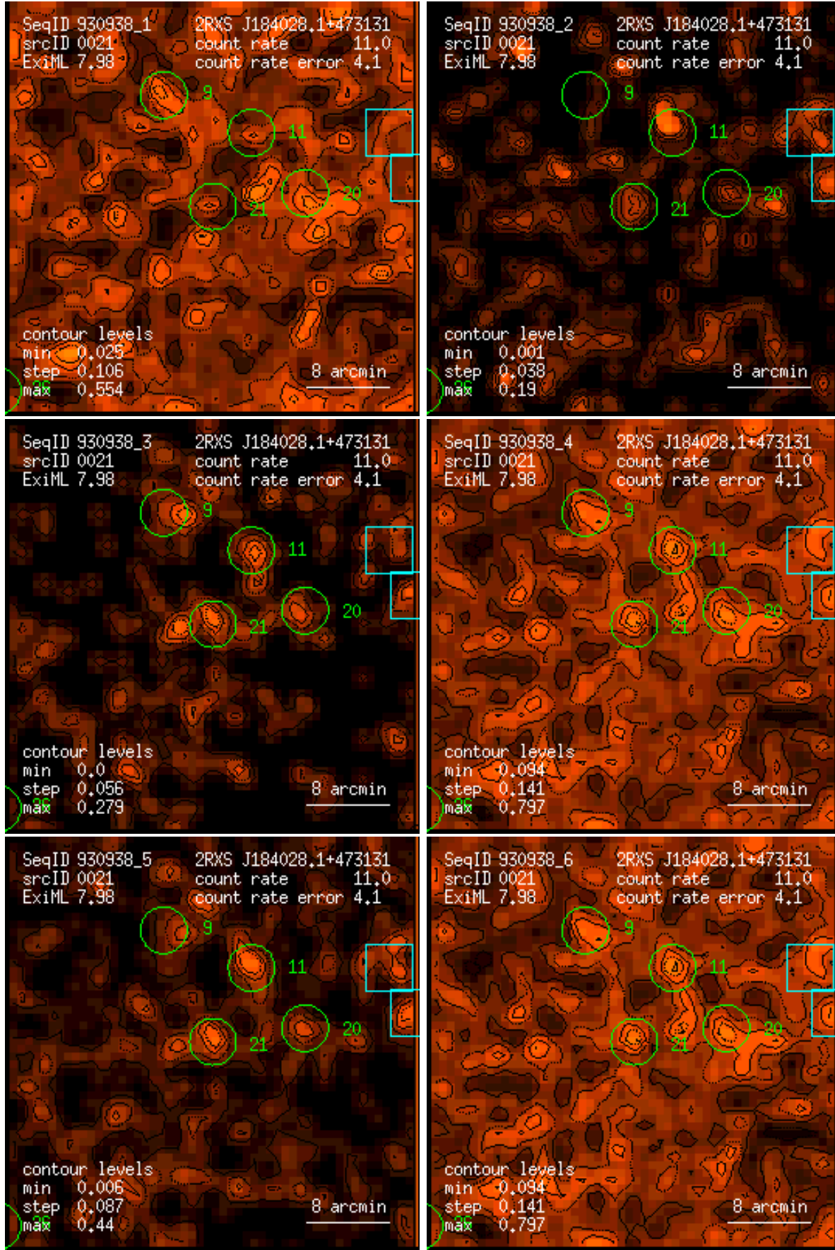
Figure 21: RASS 930938: detection 0021: band rate images, Gaussian filter: (1) PSPC channels 11 – 41, (2) 52 – 90, (3) 91 – 201, (4) 11 – 235, (5) 52 – 201, (6) 11 – 201. Broad band rates in counts/ks. Band rate contour levels in counts/ks/arcmin 2 .
