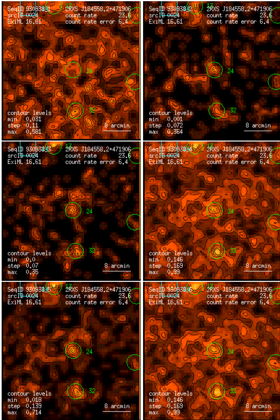
Figure 24: RASS 930938: detection 0024: band rate images, Gaussian filter: (1) PSPC channels 11 – 41, (2) 52 – 90, (3) 91 – 201, (4) 11 – 235, (5) 52 – 201, (6) 11 – 201. Broad band rates in counts/ks. Band rate contour levels in counts/ks/arcmin 2 .
