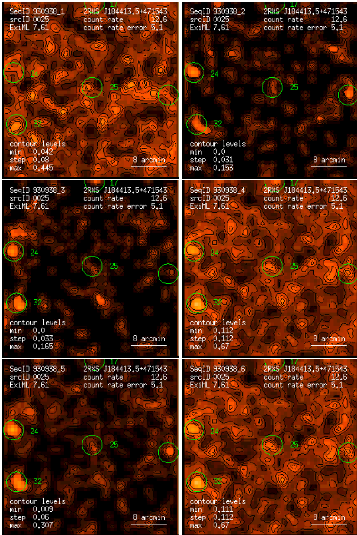
Figure 25: RASS 930938: detection 0025: band rate images, Gaussian filter: (1) PSPC channels 11 – 41, (2) 52 – 90, (3) 91 – 201, (4) 11 – 235, (5) 52 – 201, (6) 11 – 201. Broad band rates in counts/ks. Band rate contour levels in counts/ks/arcmin 2 .
