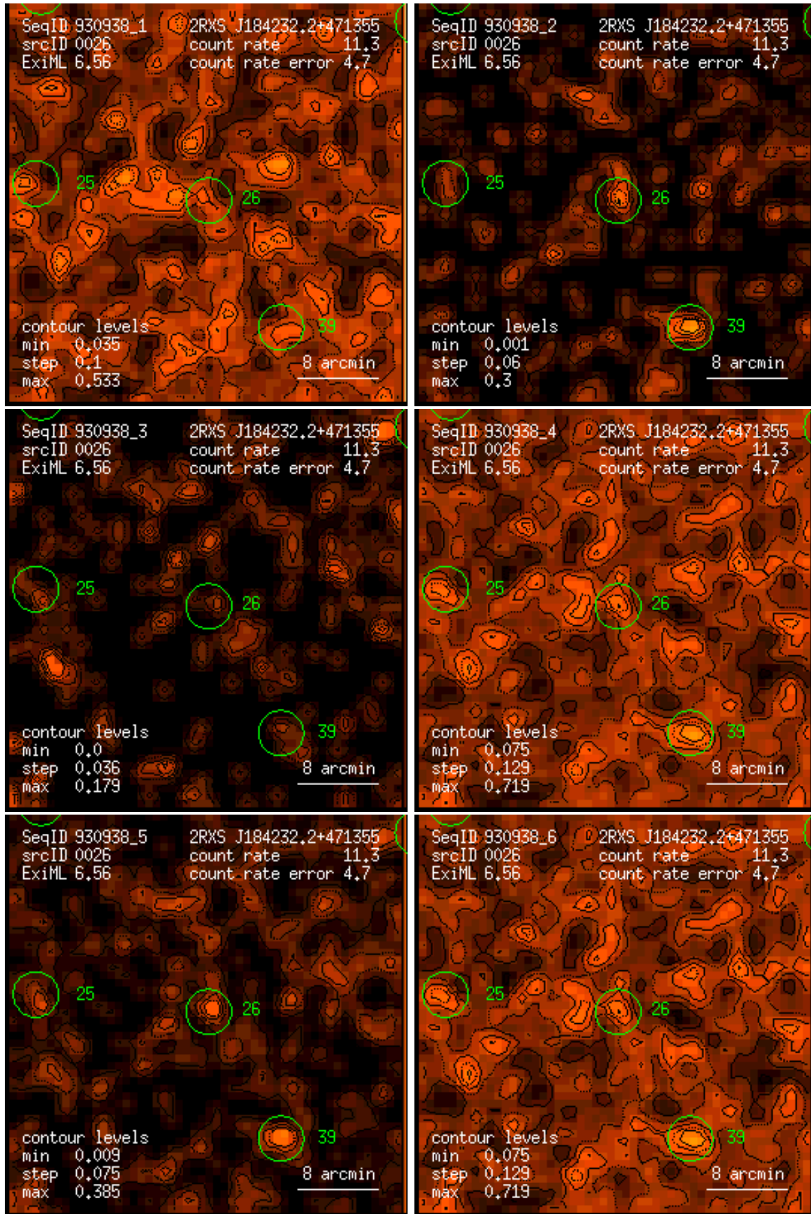
Figure 26: RASS 930938: detection 0026: band rate images, Gaussian filter: (1) PSPC channels 11 – 41, (2) 52 – 90, (3) 91 – 201, (4) 11 – 235, (5) 52 – 201, (6) 11 – 201. Broad band rates in counts/ks. Band rate contour levels in counts/ks/arcmin 2 .
